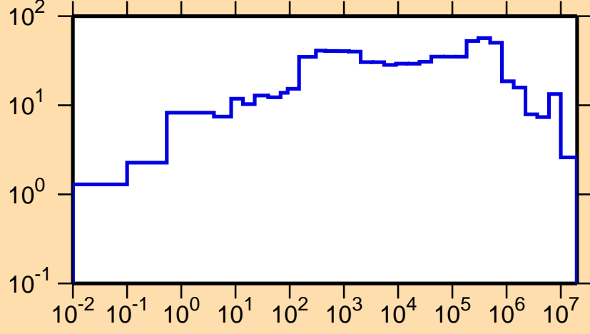
\Delta\sigma/\sigma vs. E for ^{235}\text{Pu}(n,tot.)
