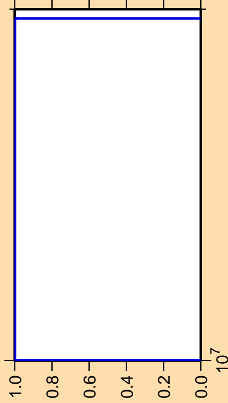
\Delta\sigma/\sigma vs. E for ^{235}\text{Pu}(\text{mt } 45)
