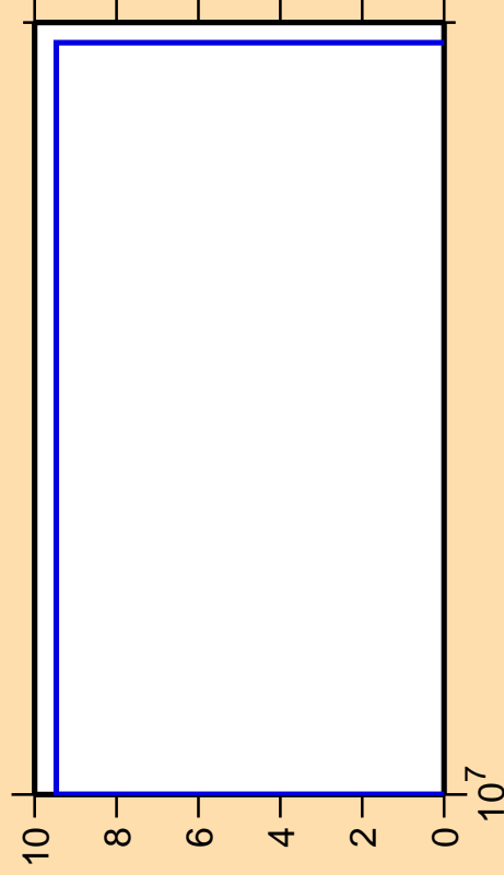
\Delta\sigma/\sigma vs. E for ^{235}\text{Pu}(\text{mt117})
