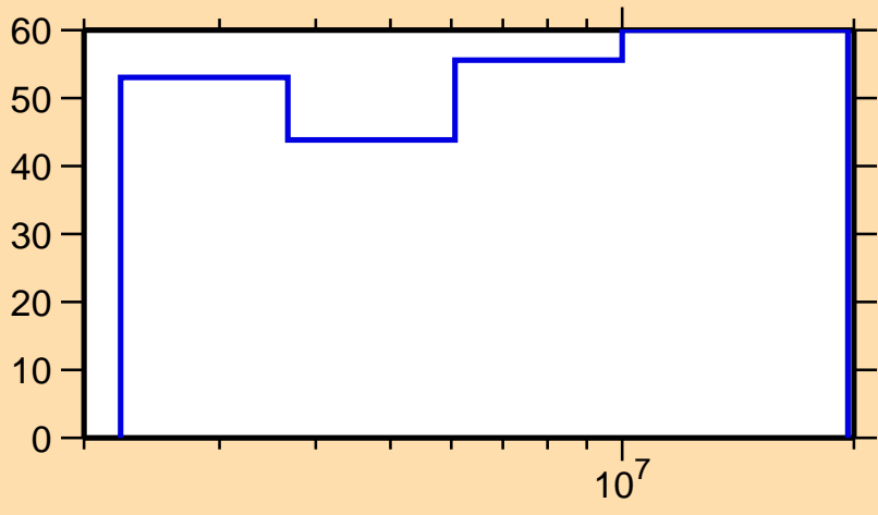
\Delta\sigma/\sigma vs. E for ^{235}\text{Pu}(n,n_1)
