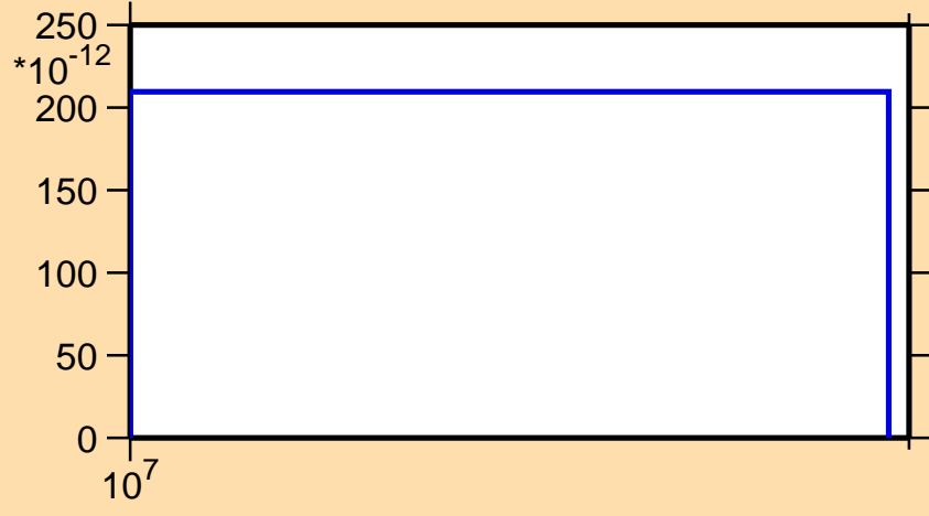
\sigma vs. E for ^{235}\text{Pu}(n,3n\alpha)
