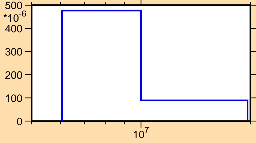
\sigma vs. E for ^{235}\text{Pu}(n,2n)
