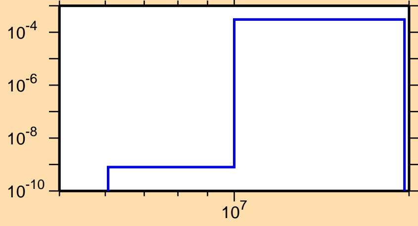
\sigma vs. E for ^{235}\text{Pu}(n,d)
