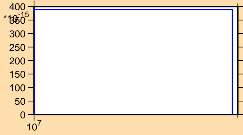
\sigma vs. E for ^{235}\text{Pu}(\text{mt } 45)
