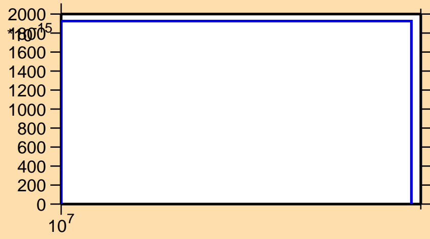
\sigma vs. E for ^{235}\text{Pu}(\text{mt117})
