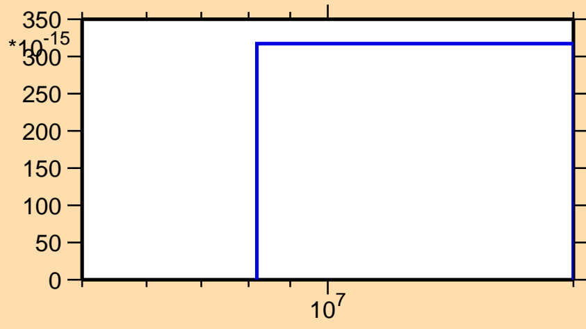
\sigma vs. E for ^{235}\text{Pu}(\text{mt } 45)
