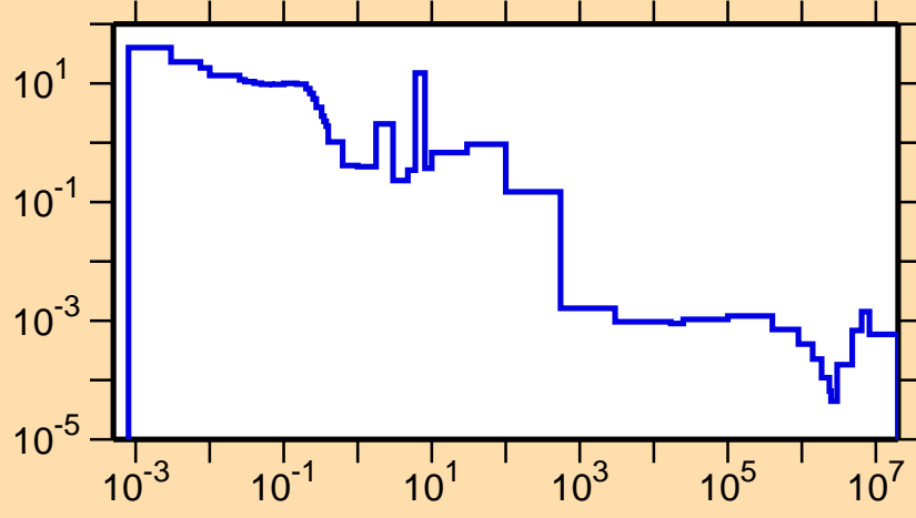
\sigma vs. E for ^{235}\text{Pu}(n,\gamma)
