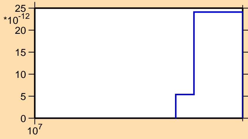
\sigma vs. E for ^{236}\text{Pu} (mt 45)
