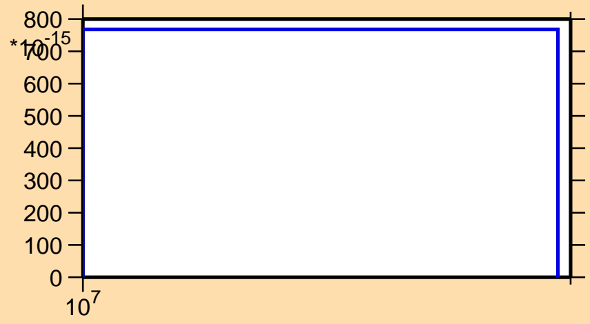
\sigma vs. E for ^{236}\text{Pu} (mt 45)
