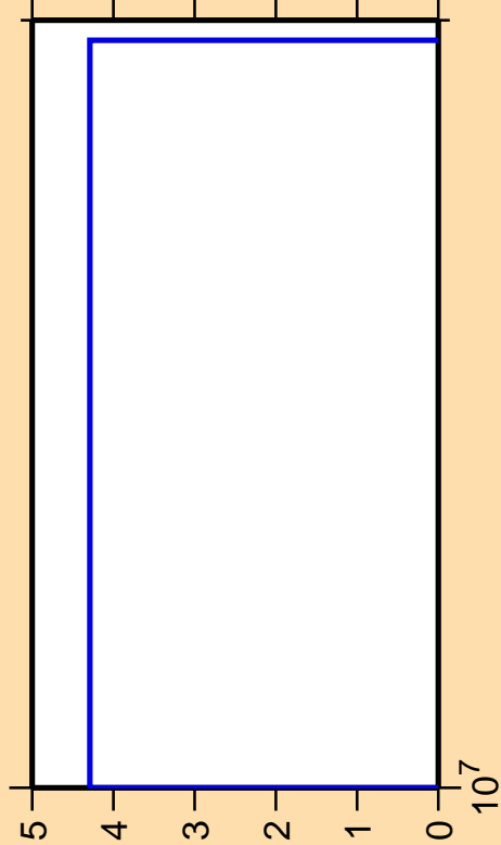
\Delta\sigma/\sigma vs. E for ^{236}\text{Pu} (mt 45)
