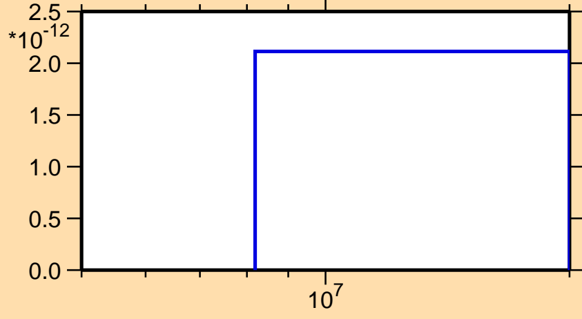
\sigma vs. E for ^{236}\text{Pu}(\text{mt117})
