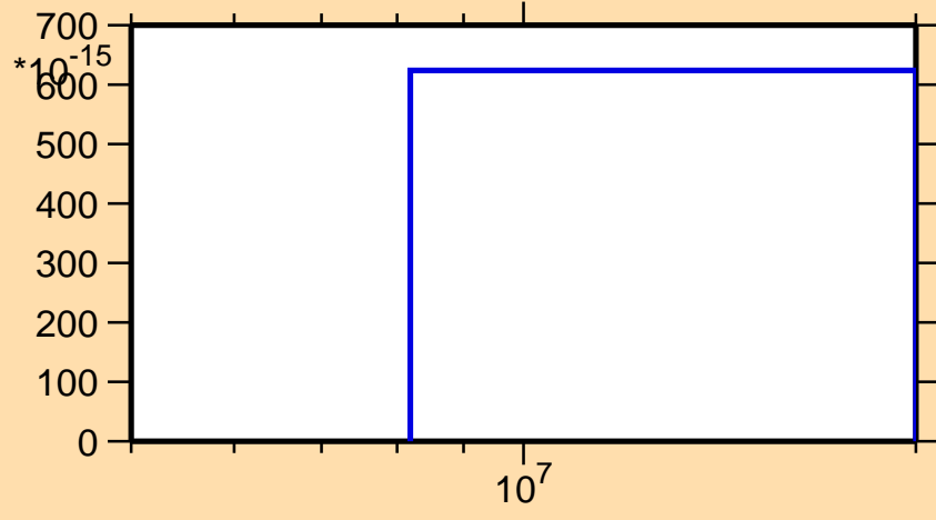
\sigma vs. E for ^{236}\text{Pu}(\text{mt } 45)
