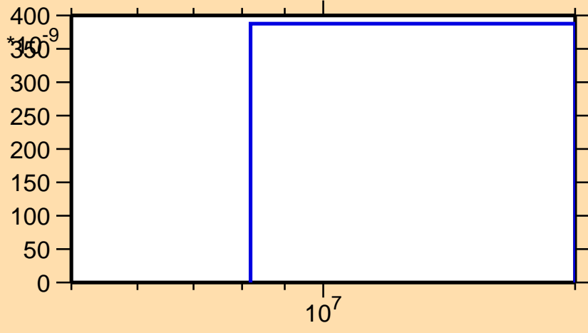
\sigma vs. E for ^{236}\text{Pu}(n,2n\alpha)
