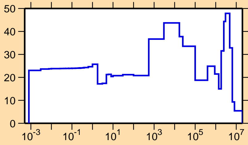
\Delta\sigma/\sigma vs. E for ^{236}\text{Pu}(n,el.)
