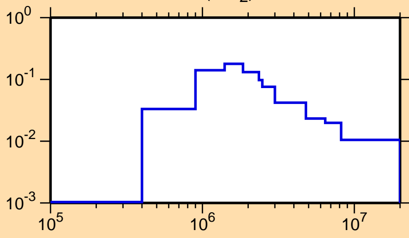
\sigma vs. E for ^{236}\text{Pu}(n,n_2)
