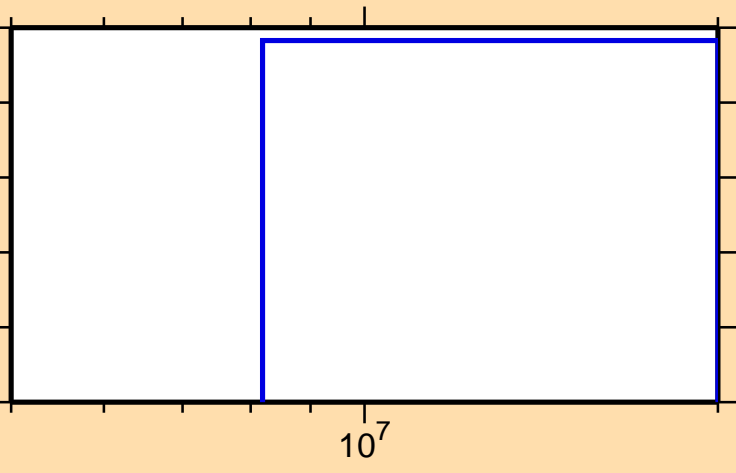
\sigma vs. E for ^{236}\text{Pu}(n,3n)
