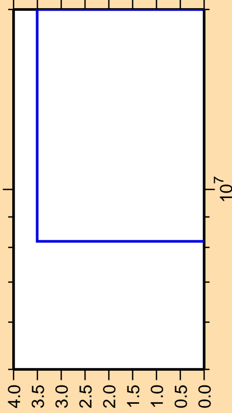
\Delta\sigma/\sigma vs. E for ^{236}\text{Pu}(\text{mt } 45)
