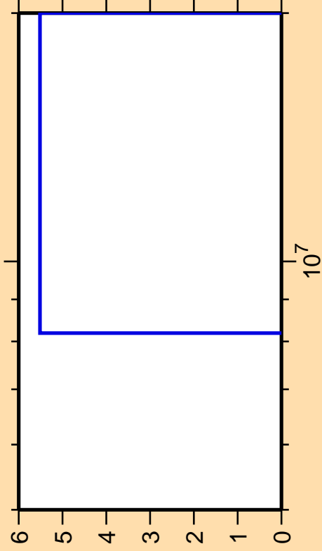
\Delta\sigma/\sigma vs. E for ^{236}\text{Pu}(n,3n\alpha)
