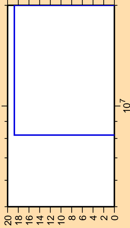
\Delta\sigma/\sigma vs. E for ^{236}\text{Pu}(\text{mt117})
