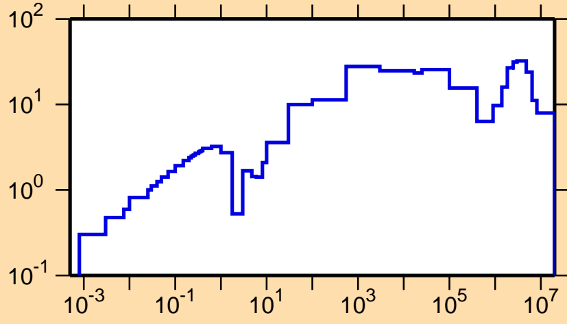
\Delta\sigma/\sigma vs. E for ^{236}\text{Pu}(n,tot.)
