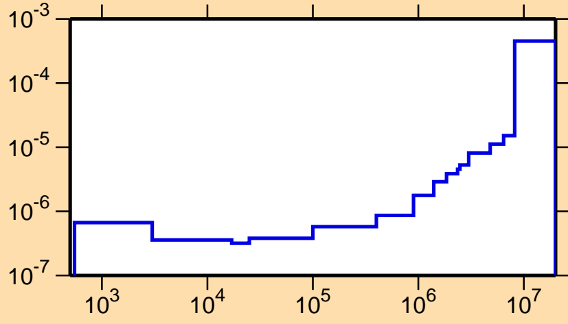
\sigma vs. E for ^{236}\text{Pu}(n,\alpha)
