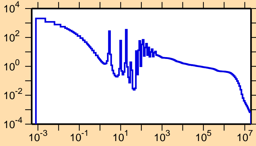
\sigma vs. E for ^{238}\text{Pu}(n,\gamma)
