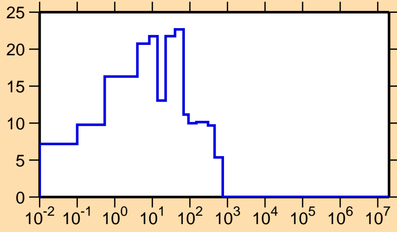
\Delta\sigma/\sigma vs. E for ^{238}\text{Pu}(n,\text{el.})
