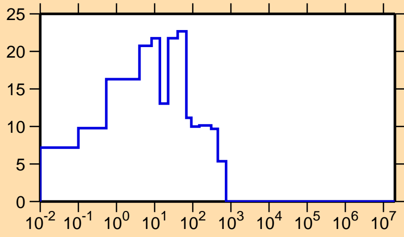
\Delta\sigma/\sigma vs. E for ^{238}\text{Pu}(n,el.)
