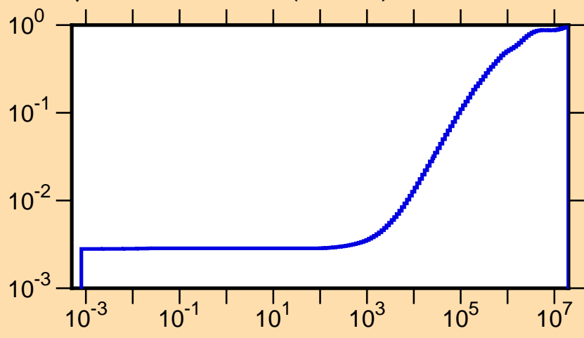
\mu vs. E for ^{240}\text{Pu}(\text{mt251})
