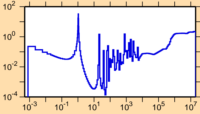
\sigma vs. E for ^{240}\text{Pu}(n,f)
