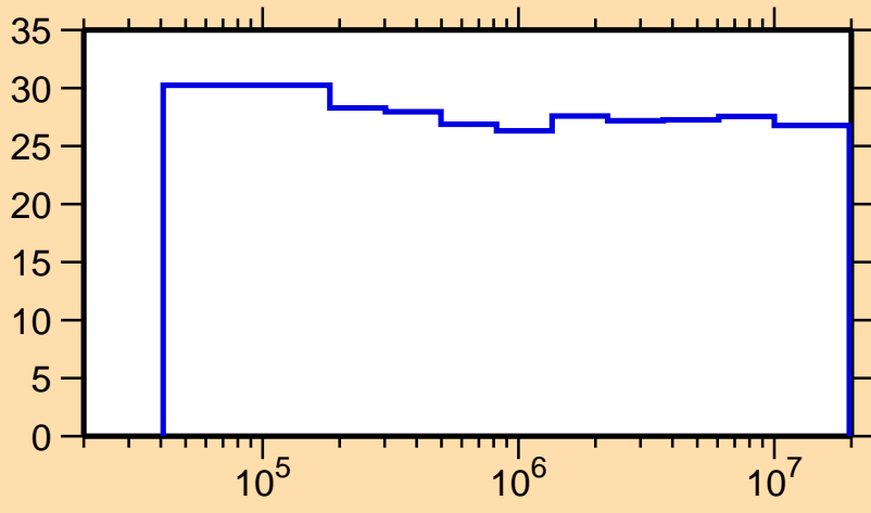
\Delta\sigma/\sigma vs. E for ^{240}\text{Pu}(n,n_1)
