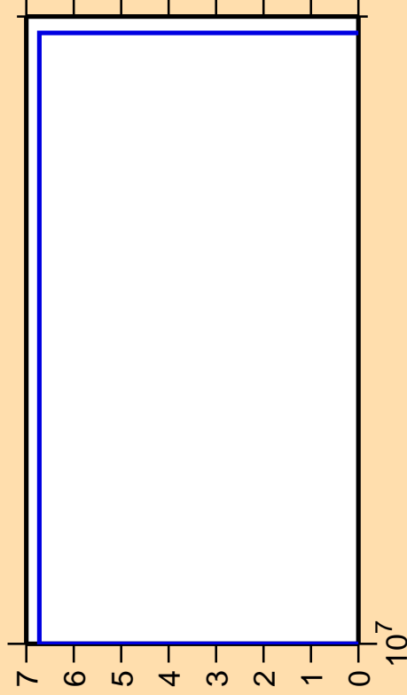
\Delta\sigma/\sigma vs. E for ^{240}\text{Pu}(n,3n\alpha)
