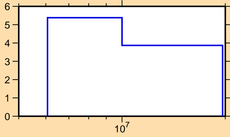
Δσ/σ vs. E for ^{240}\text{Pu}(n,\text{nonel.})
