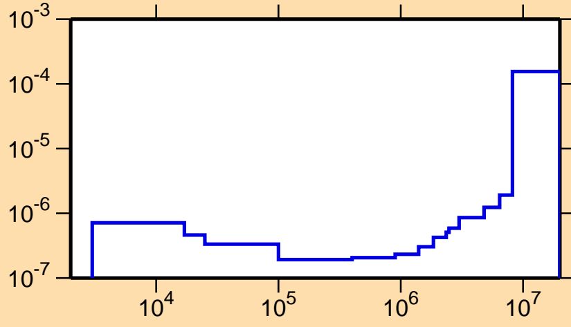
\sigma vs. E for ^{240}\text{Pu}(n,\alpha)
