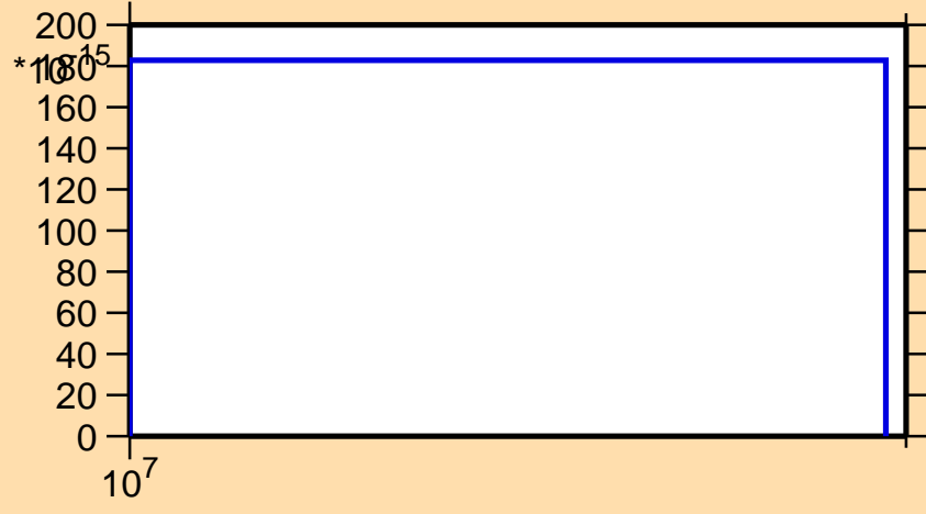
\sigma vs. E for ^{241}\text{Pu}(n,\text{He3})
