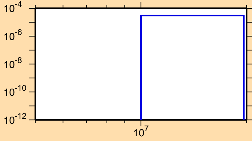
\sigma vs. E for ^{241}\text{Pu}(n,t)
