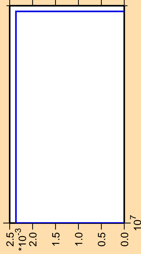
\Delta\sigma/\sigma vs. E for ^{241}\text{Pu}(n,\text{He3})
