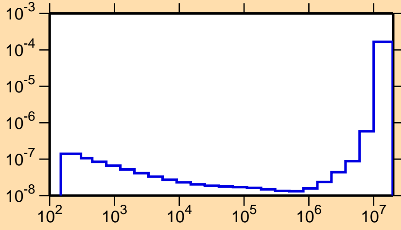
\sigma vs. E for ^{241}\text{Pu}(n,\alpha)
