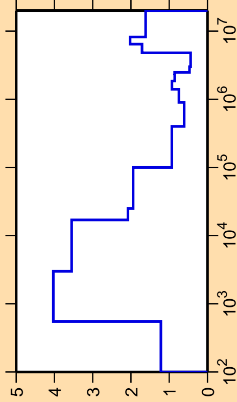
\Delta\sigma/\sigma vs. E for ^{241}\text{Pu}(n,\text{nonel.})
