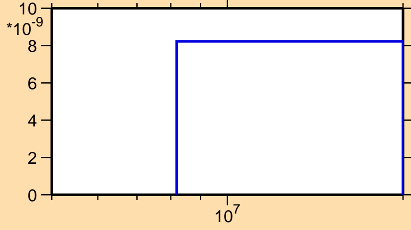
\sigma vs. E for ^{241}\text{Pu}(n,nd)
