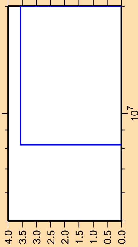
\Delta\sigma/\sigma vs. E for ^{241}\text{Pu}(n,nd)
