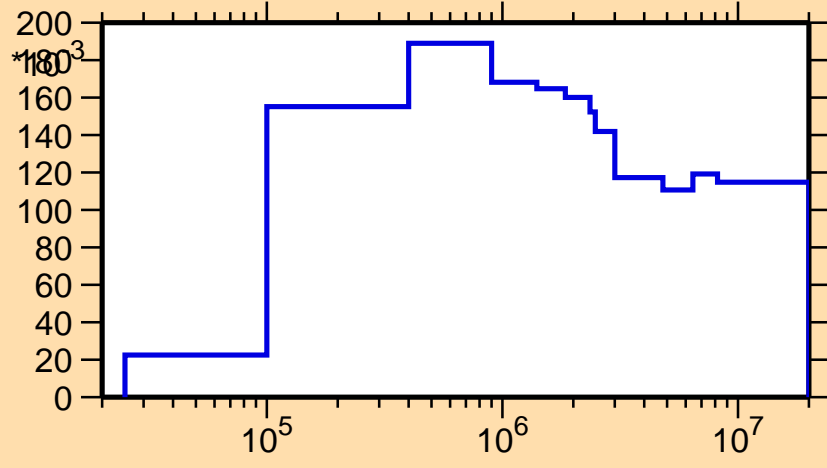
\sigma vs. E for ^{241}\text{Pu}(n,n_1)
