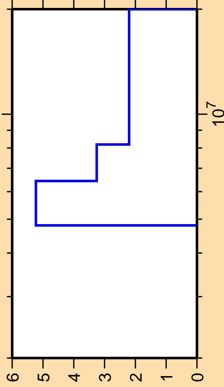
\Delta\sigma/\sigma vs. E for ^{241}\text{Pu}(n,n\text{cont.})
