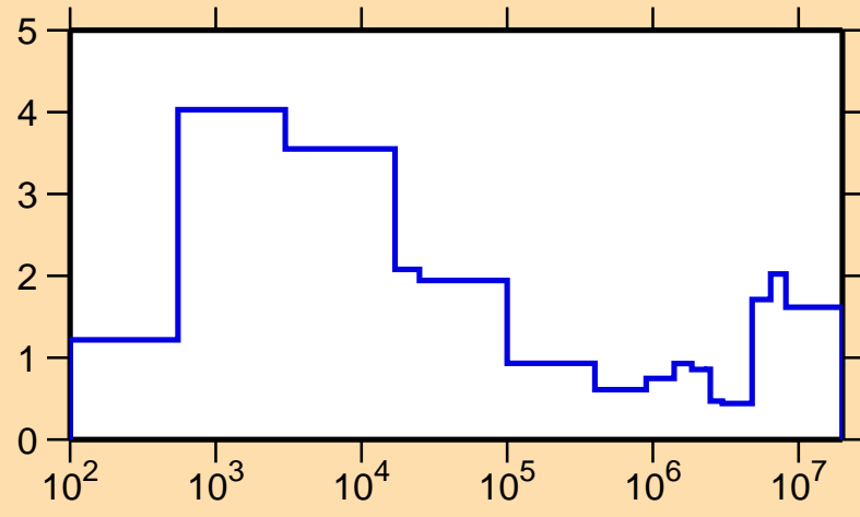
\Delta\sigma/\sigma vs. E for ^{241}\text{Pu}(n,\text{nonel.})
