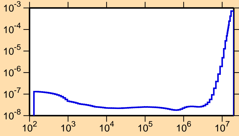
\sigma vs. E for ^{243}\text{Pu}(n,\alpha)
