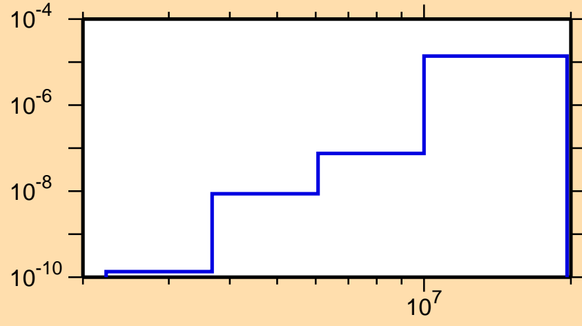
\sigma vs. E for ^{243}\text{Pu}(n,n\alpha)
