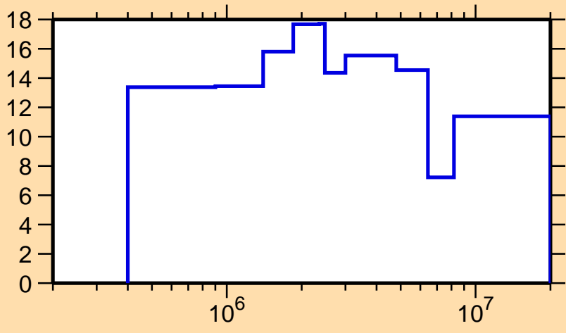
\Delta\sigma/\sigma vs. E for ^{243}\text{Pu}(n,\text{tot.})
