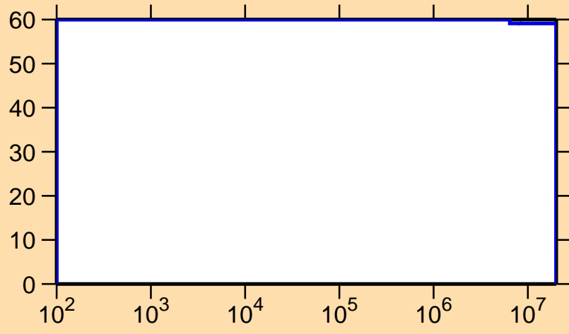
\Delta\sigma/\sigma vs. E for ^{243}\text{Pu}(n,f)
