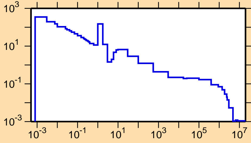
\sigma vs. E for ^{243}\text{Pu}(n,\gamma)
