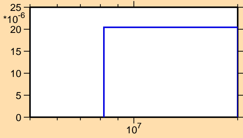
\sigma vs. E for ^{243}\text{Pu}(n,t)
