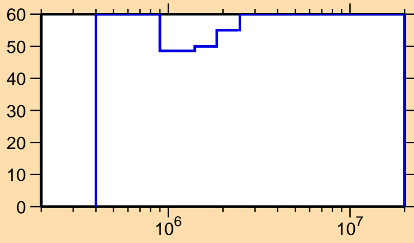
\Delta\sigma/\sigma vs. E for ^{243}\text{Pu}(n,n\text{cont.})
