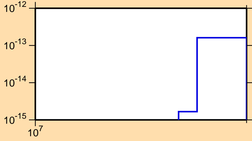
\sigma vs. E for ^{244}\text{Pu}(n,\text{He}3)
