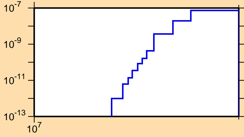
\sigma vs. E for ^{244}\text{Pu}(n,3n\alpha)
