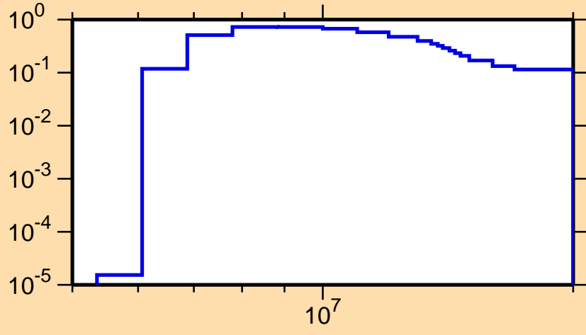
\sigma vs. E for ^{244}\text{Pu}(n,2n)
