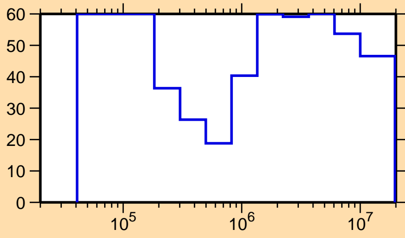
\Delta\sigma/\sigma vs. E for ^{244}\text{Pu}(n,\text{nonel.})
