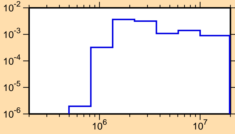
\sigma vs. E for ^{244}\text{Pu}(n,n_4)
