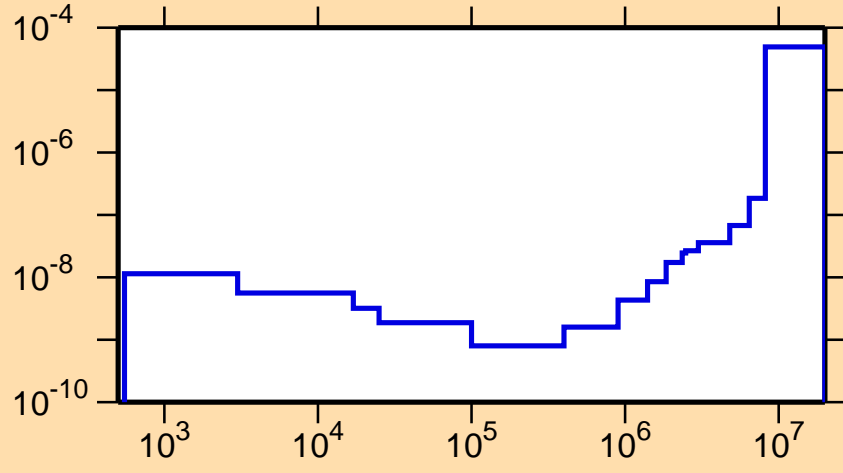
\sigma vs. E for ^{244}\text{Pu}(n,\alpha)
