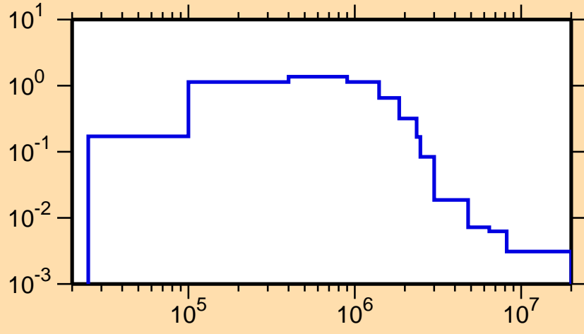
\sigma vs. E for ^{244}\text{Pu}(n,n_1)
