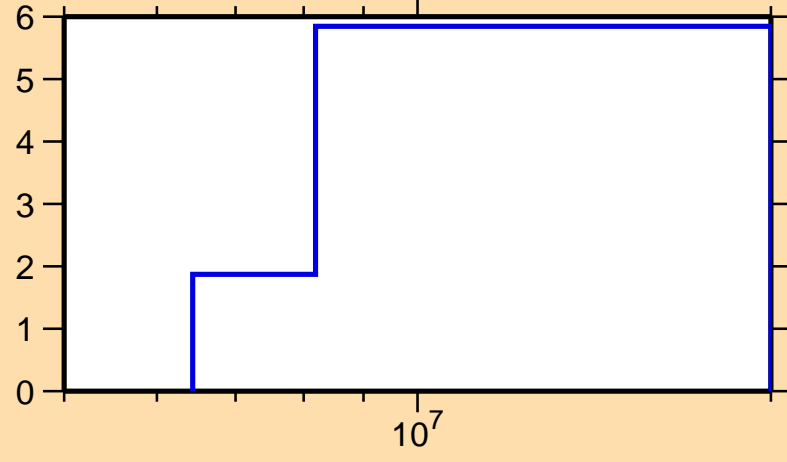
\Delta\sigma/\sigma vs. E for ^{244}\text{Pu}(n,\text{el.})
