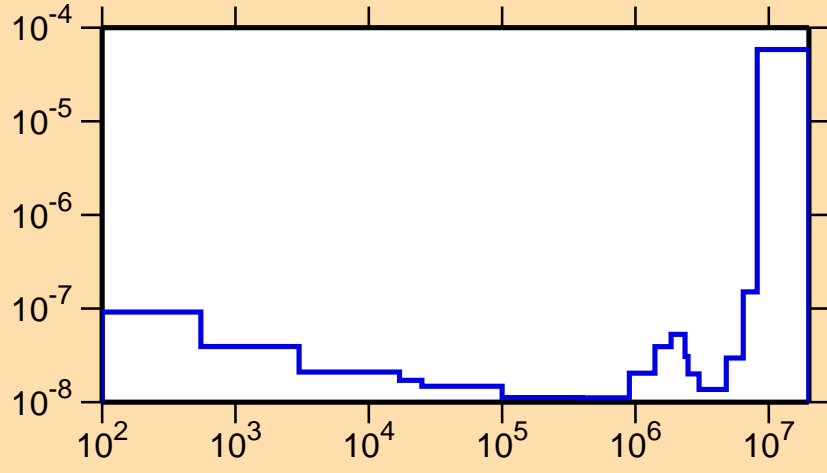
\sigma vs. E for ^{245}\text{Pu}(n,\alpha)
