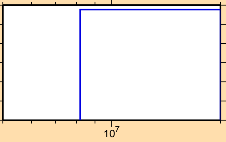
\sigma vs. E for ^{245}\text{Pu}(n,nt)
