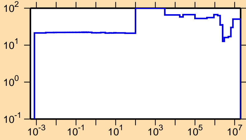
\Delta\sigma/\sigma vs. E for ^{245}\text{Pu}(n,el.)
