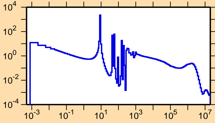
\sigma vs. E for ^{246}\text{Pu}(n,\gamma)
