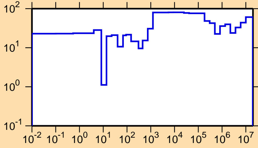
\Delta\sigma/\sigma vs. E for ^{246}\text{Pu}(n,el.)
