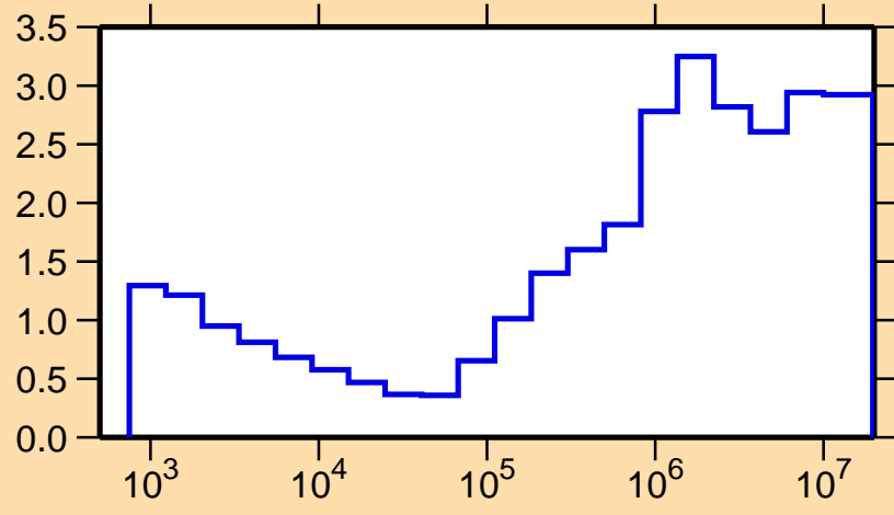
\sigma vs. E for ^{246}\text{Pu}(n,\text{nonel.})
