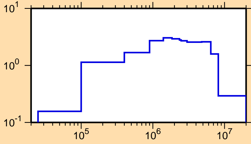
\sigma vs. E for ^{246}\text{Pu}(n,\text{inel.})
