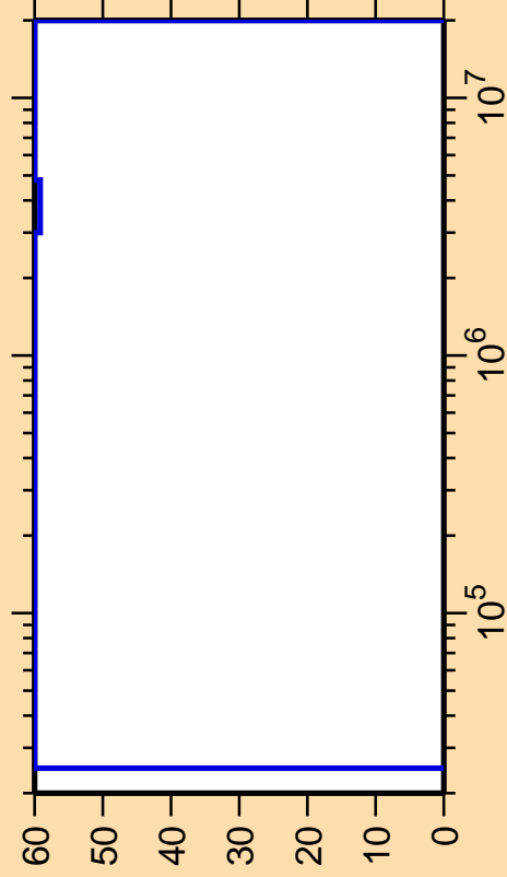
\Delta\sigma/\sigma vs. E for ^{246}\text{Pu}(n,\text{inel.})
