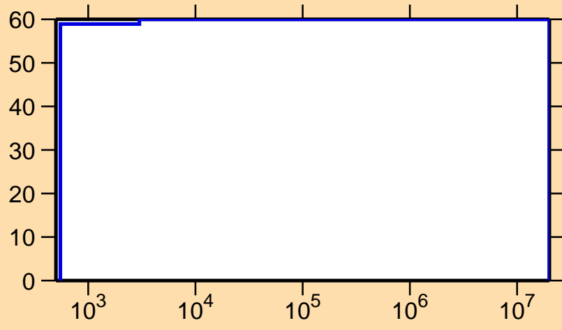
\Delta\sigma/\sigma vs. E for ^{246}\text{Pu}(n,\gamma)
