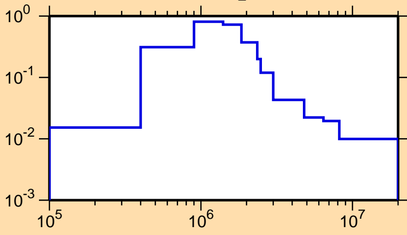
\sigma vs. E for ^{246}\text{Pu}(n,n_2)
