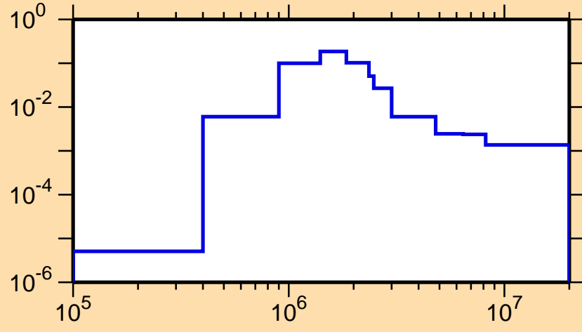
\sigma vs. E for ^{246}\text{Pu}(n,n_3)
