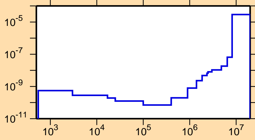
\sigma vs. E for ^{246}\text{Pu}(n,\alpha)
