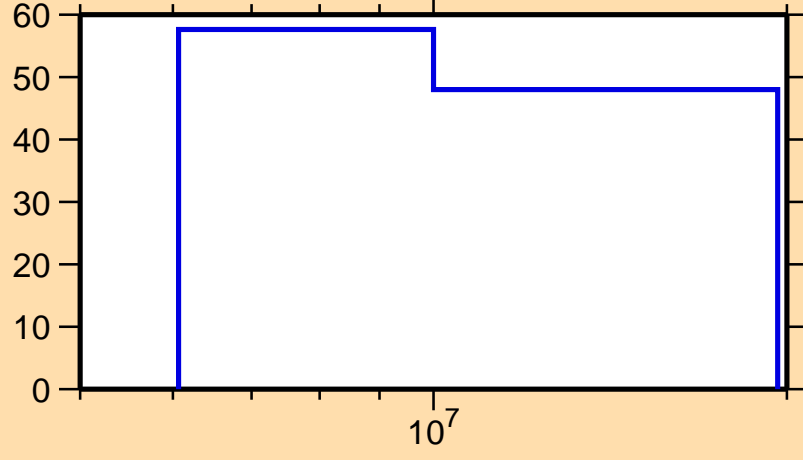
\Delta\sigma/\sigma vs. E for ^{247}\text{Pu}(n,el.)
