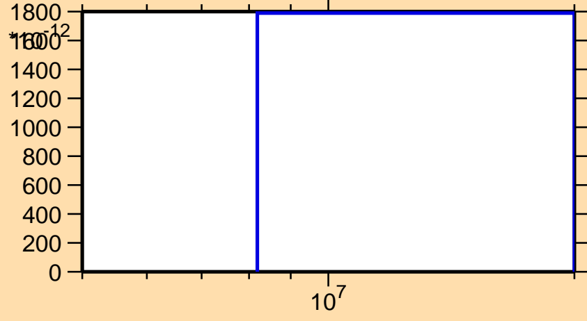
\sigma vs. E for ^{247}\text{Pu}(n,nd)
