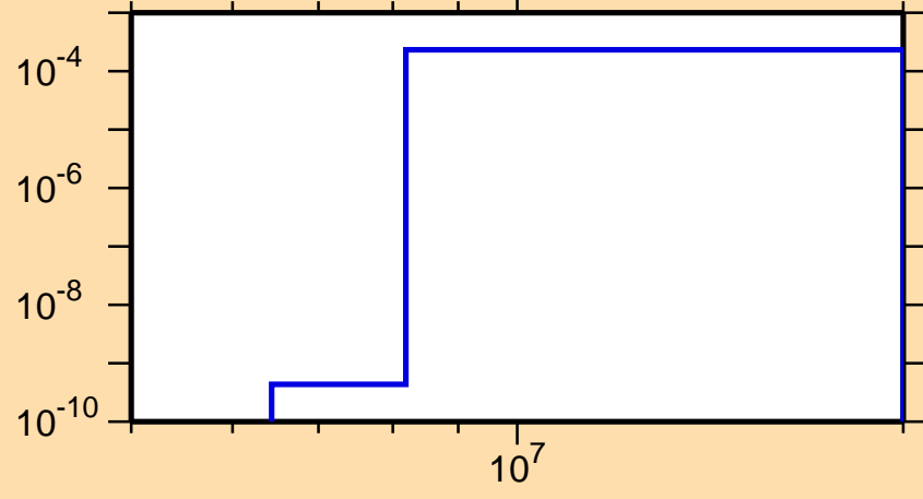
\sigma vs. E for ^{247}\text{Pu}(n,p)
