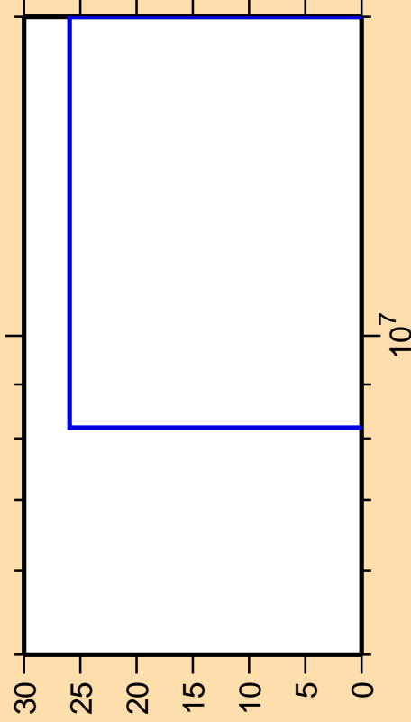
\Delta\sigma/\sigma vs. E for ^{247}\text{Pu}(n,nd)
