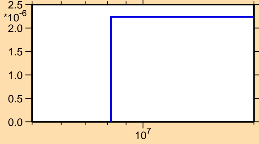
\sigma vs. E for ^{247}\text{Pu}(n,np)
