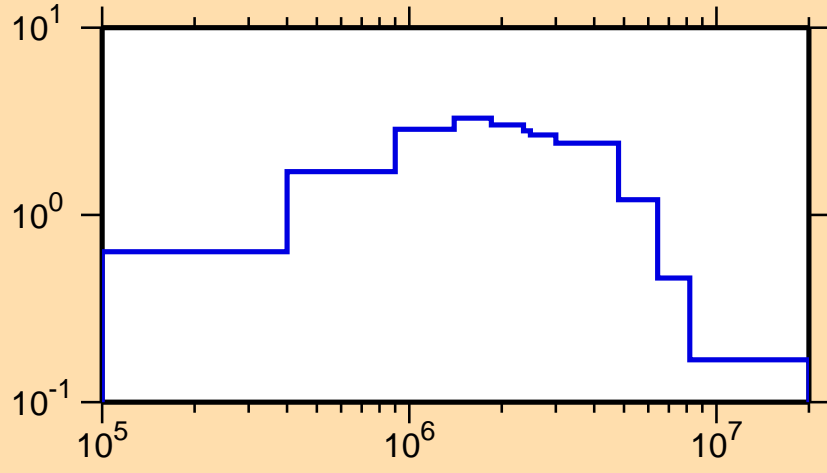
\sigma vs. E for ^{247}\text{Pu}(n,\text{inel.})
