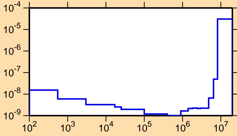
\sigma vs. E for ^{247}\text{Pu}(n,\alpha)
