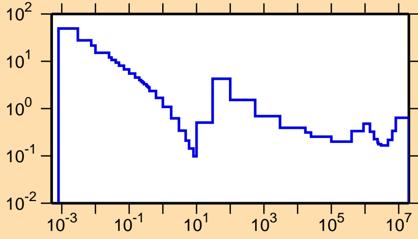
\sigma vs. E for ^{247}\text{Pu}(n,f)
