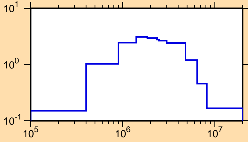
\sigma vs. E for ^{247}\text{Pu}(n,n\text{cont.})
