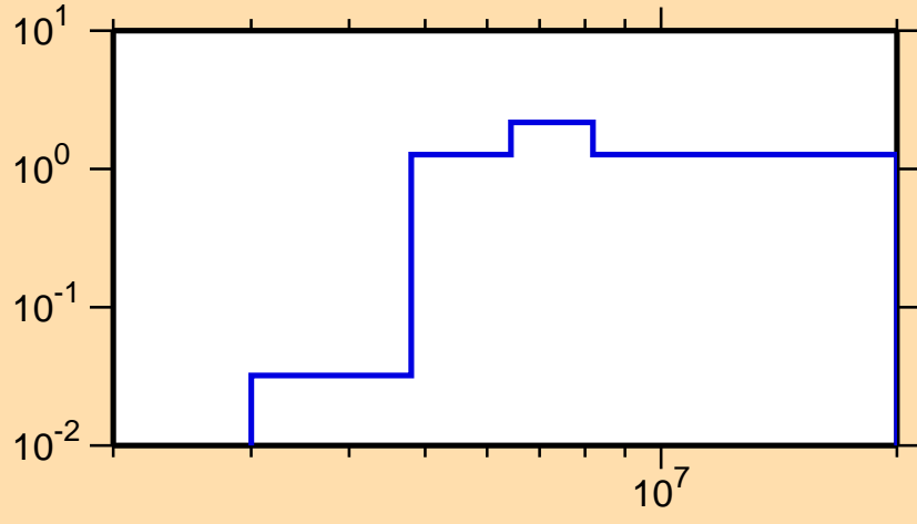
\sigma vs. E for ^{247}\text{Pu}(n,2n)
