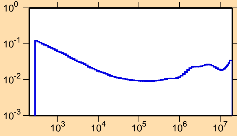
\sigma vs. E for ^{208}\text{Ra}(n,\alpha)
