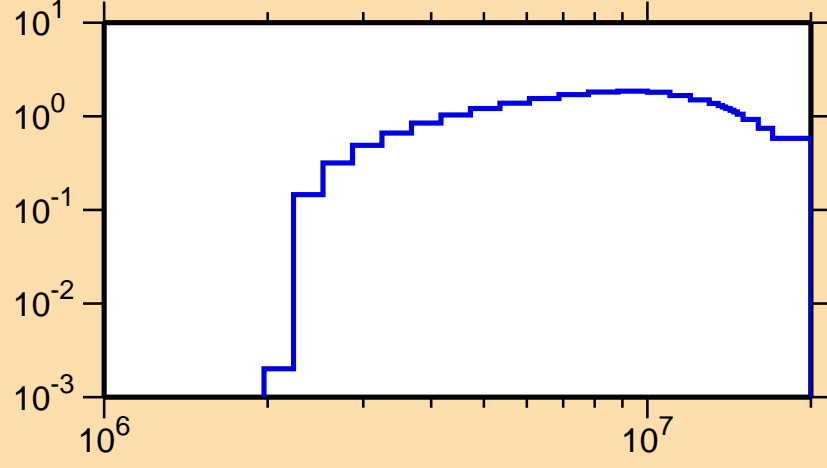
\sigma vs. E for ^{208}\text{Ra}(n,n\text{cont.})
