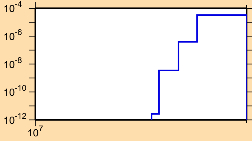
\sigma vs. E for ^{208}\text{Ra}(n,2np)
