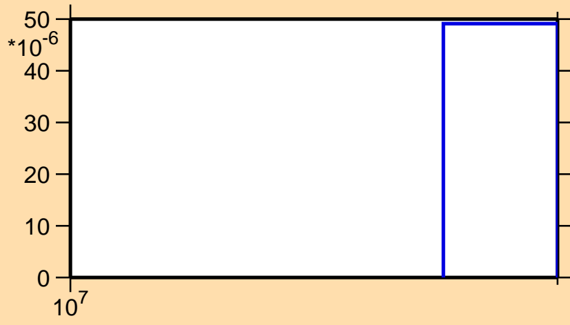
\sigma vs. E for ^{208}\text{Ra}(n,3n)
