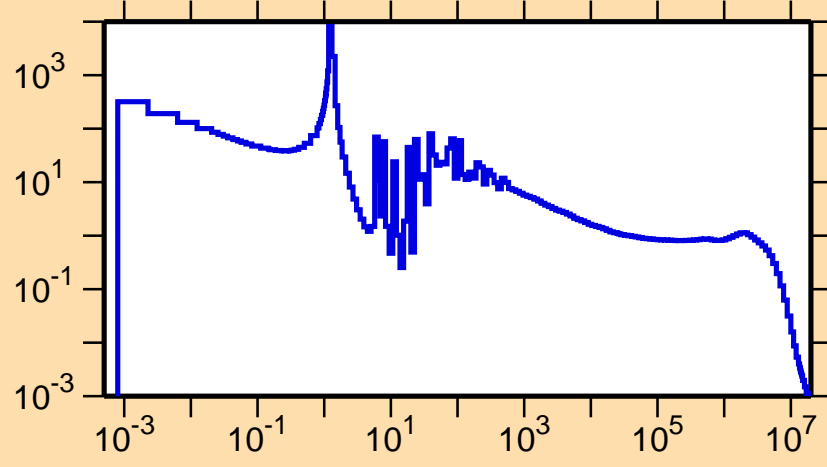
\sigma vs. E for ^{208}\text{Ra}(n,\gamma)
