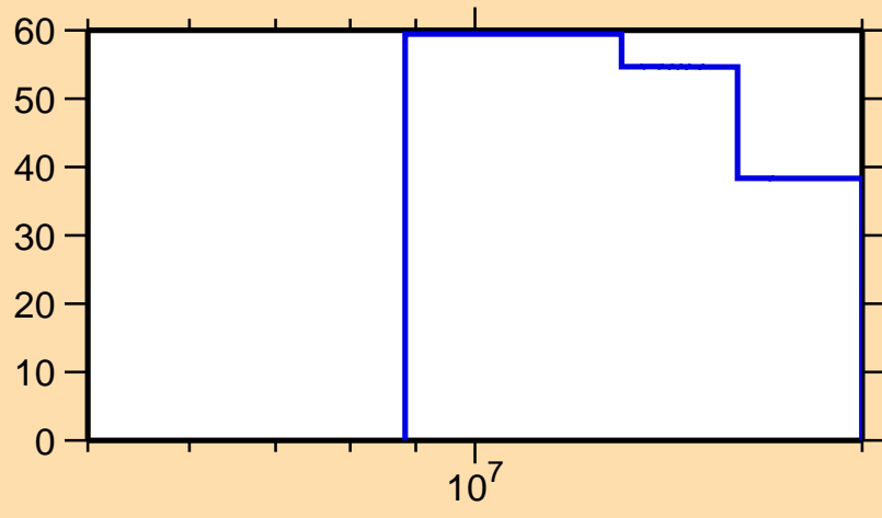
\Delta\sigma/\sigma vs. E for ^{208}\text{Ra}(n,2n)
