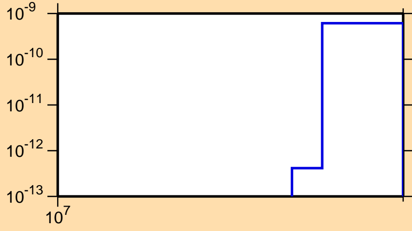
\sigma vs. E for ^{208}\text{Ra}(n,nt)
