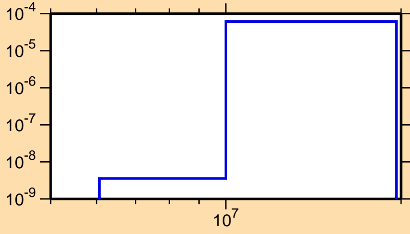
\sigma vs. E for ^{208}\text{Ra}(\text{mt117})
