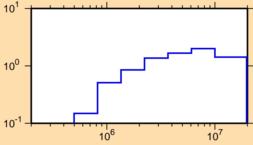
\sigma vs. E for ^{208}\text{Ra}(n,\text{inel.})
