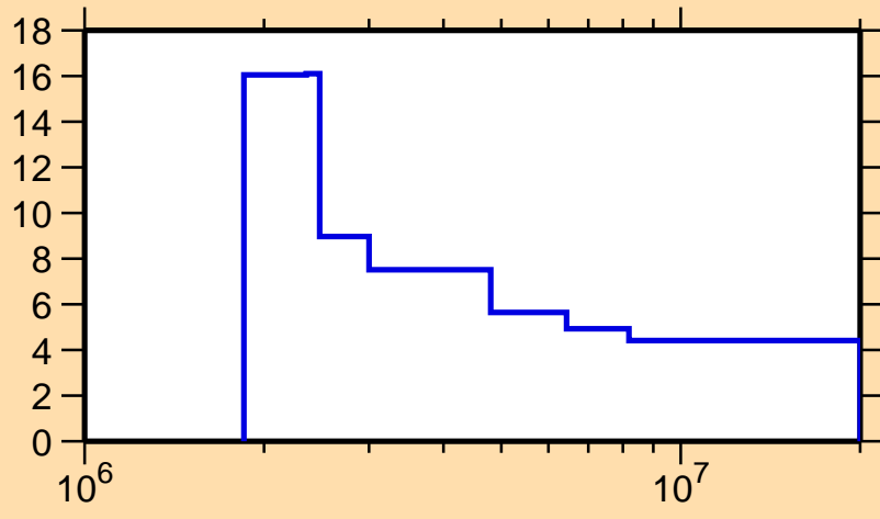
\Delta\sigma/\sigma vs. E for ^{208}\text{Ra}(n,\text{nonel.})
