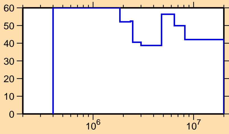
\Delta\sigma/\sigma vs. E for ^{208}\text{Ra}(n,n_1)
