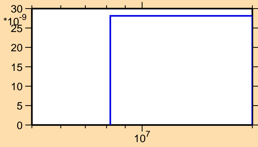
\sigma vs. E for ^{208}\text{Ra}(n,\text{pd})
