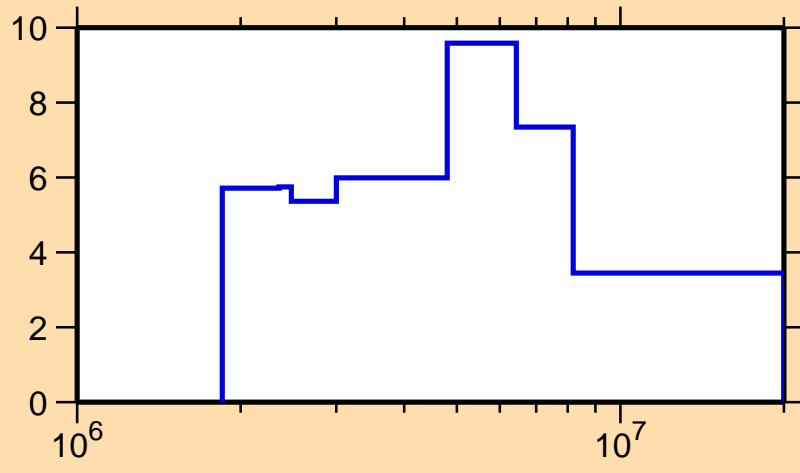
\Delta\sigma/\sigma vs. E for ^{208}\text{Ra}(n,\text{tot.})
