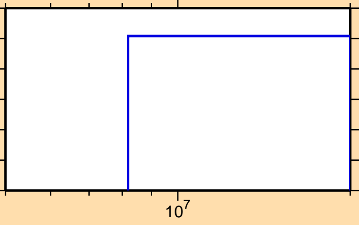
\sigma vs. E for ^{208}\text{Ra}(n,t)
