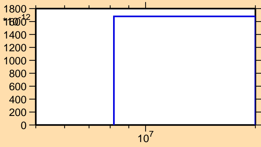
\sigma vs. E for ^{208}\text{Ra}(n,\text{nd})
