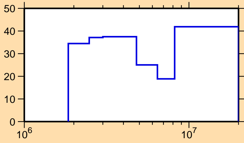
\Delta\sigma/\sigma vs. E for ^{208}\text{Ra}(n,n\text{cont.})
