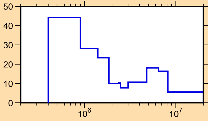
\Delta\sigma/\sigma vs. E for ^{208}\text{Ra}(n,\text{el.})
