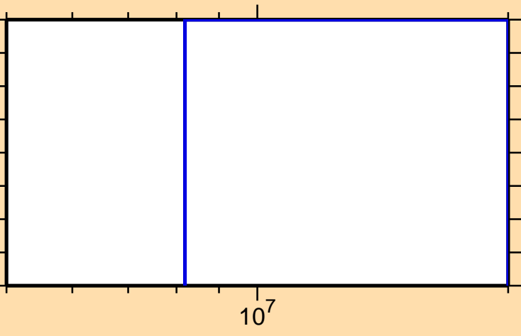
\sigma vs. E for ^{208}\text{Ra}(n,3n)
