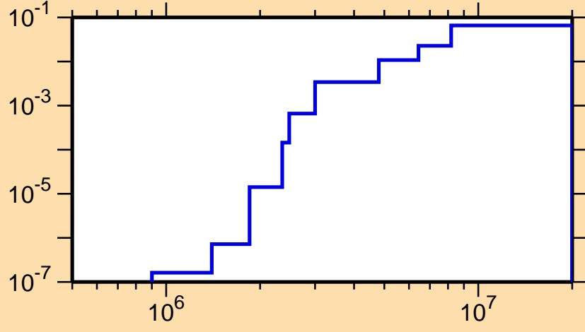
\sigma vs. E for ^{208}\text{Ra}(n,n\alpha)
