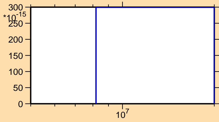
\sigma vs. E for ^{208}\text{Ra}(n,3n\alpha)
