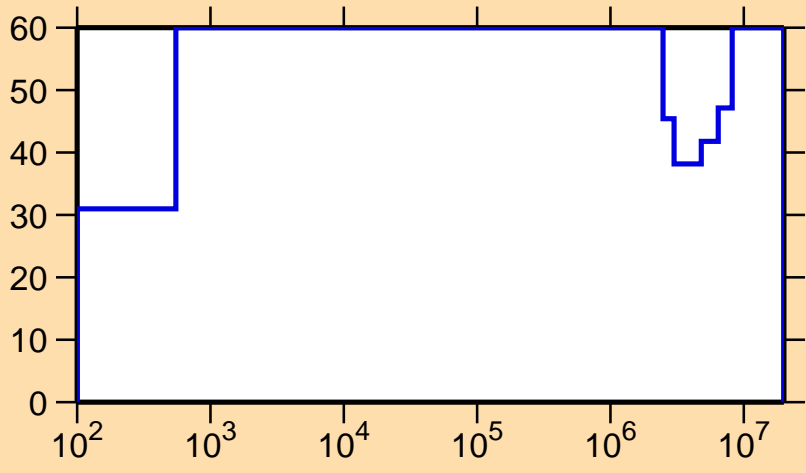
\Delta\sigma/\sigma vs. E for ^{208}\text{Ra}(n,p)
