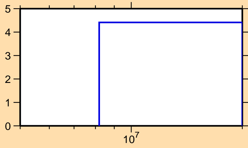
\Delta\sigma/\sigma vs. E for ^{208}\text{Ra}(n,\text{nonel.})
