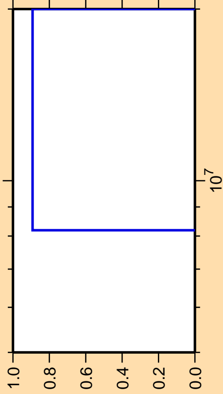
\Delta\sigma/\sigma vs. E for ^{208}\text{Ra}(n,3n\alpha)
