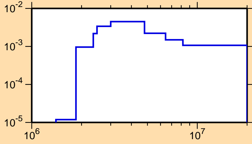
\sigma vs. E for ^{208}\text{Ra}(n,n_4)
