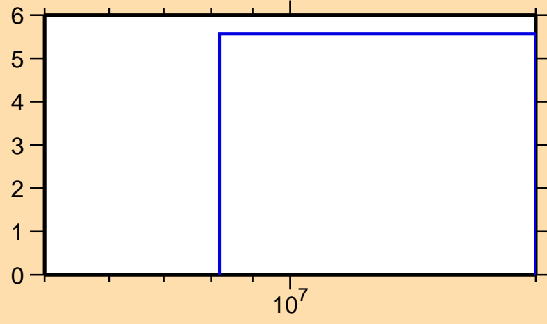
\Delta\sigma/\sigma vs. E for ^{208}\text{Ra}(n,\text{el.})
