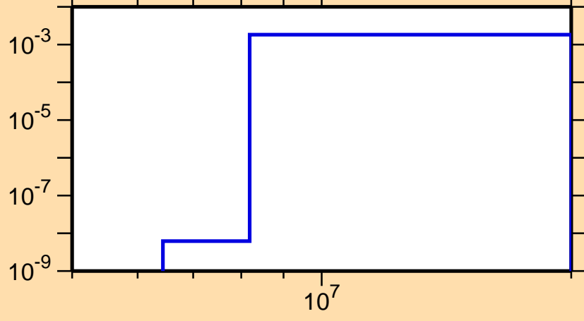
\sigma vs. E for ^{208}\text{Ra}(\text{mt } 45)
