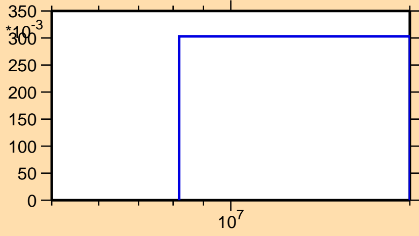
\sigma vs. E for ^{208}\text{Ra}(n,2n)
