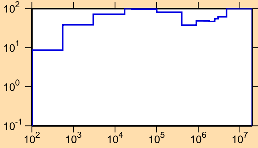
\Delta\sigma/\sigma vs. E for ^{208}\text{Ra}(n,\gamma)
