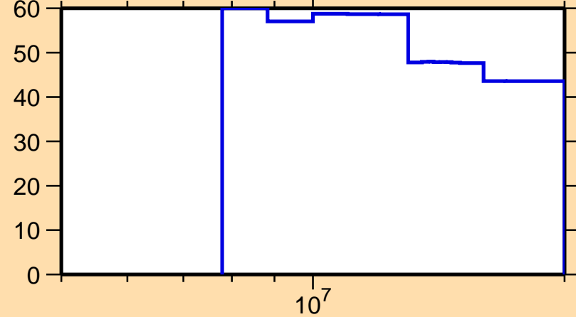
\Delta\sigma/\sigma vs. E for ^{209}\text{Ra}(n,2n)
