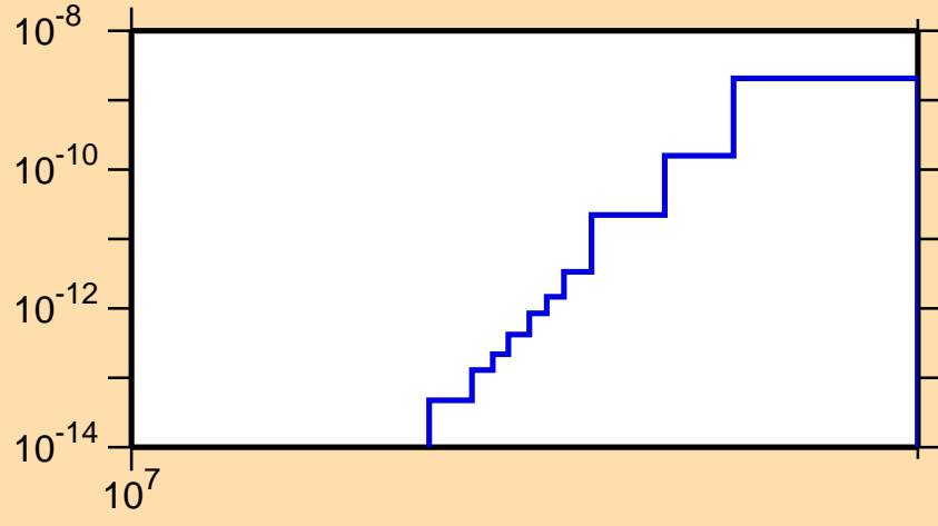
\sigma vs. E for ^{209}\text{Ra}(\text{mt } 34)
