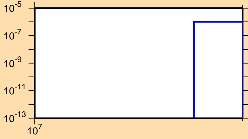
\sigma vs. E for ^{209}\text{Ra}(n,3n\alpha)
