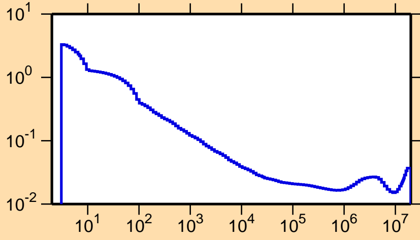
\sigma vs. E for ^{209}\text{Ra}(n,\alpha)
