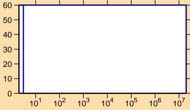
\Delta\sigma/\sigma vs. E for ^{209}\text{Ra}(n,\gamma)
