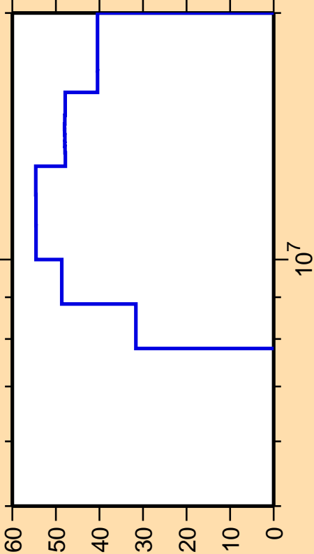
\Delta\sigma/\sigma vs. E for ^{209}\text{Ra}(n,n\text{cont.})
