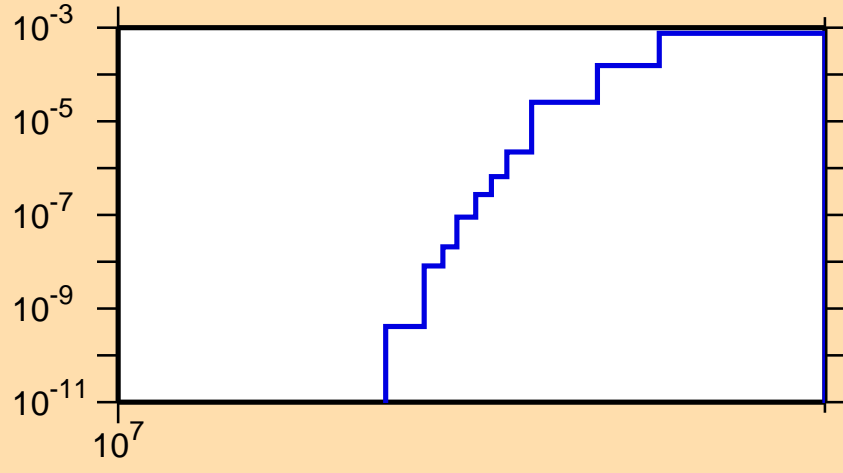
\sigma vs. E for ^{209}\text{Ra}(n,2np)
