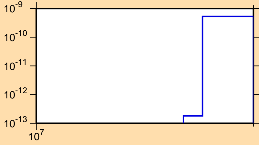
\sigma vs. E for ^{209}\text{Ra}(n,nt)
