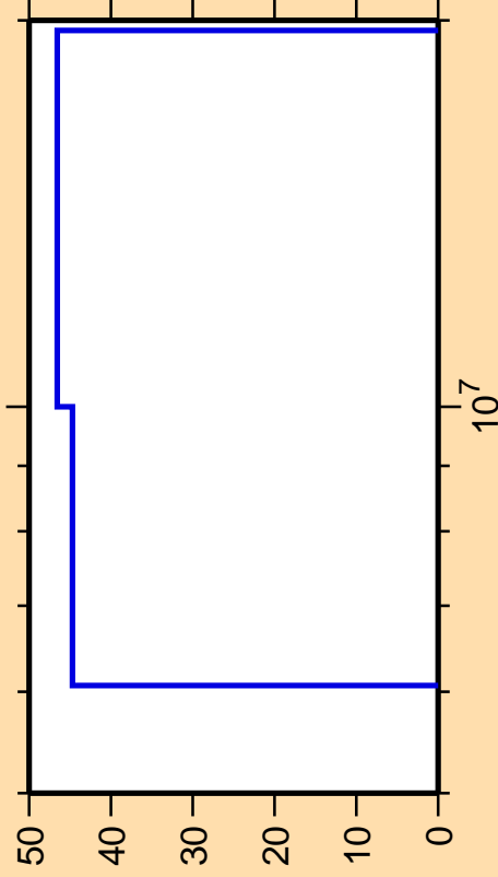
\Delta\sigma/\sigma vs. E for ^{209}\text{Ra}(n,p)
