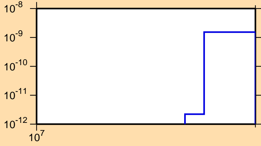
\sigma vs. E for ^{210}\text{Ra}(n,nt)
