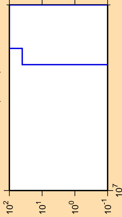
\Delta\sigma/\sigma vs. E for ^{210}\text{Ra} (mt 34)
