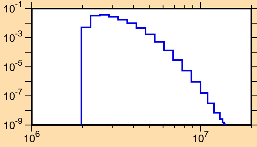
\sigma vs. E for ^{210}\text{Ra}(n,n_1)
