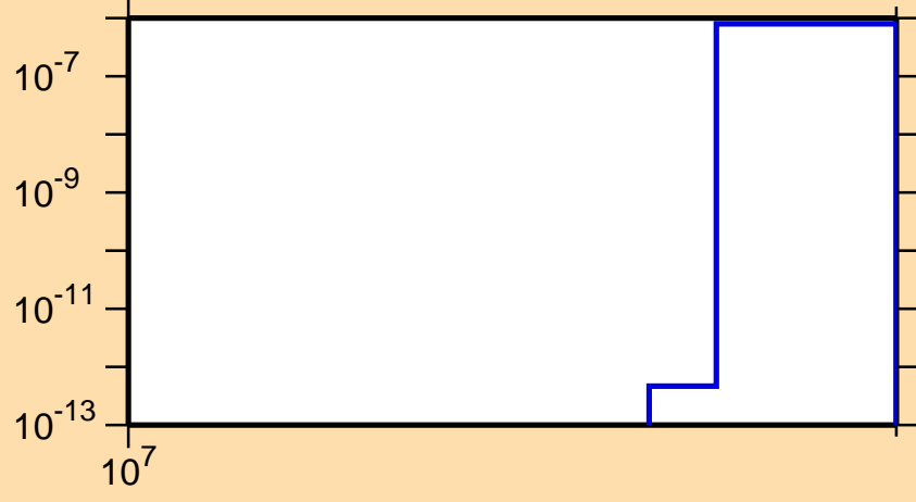
\sigma vs. E for ^{210}\text{Ra}(n,3n\alpha)
