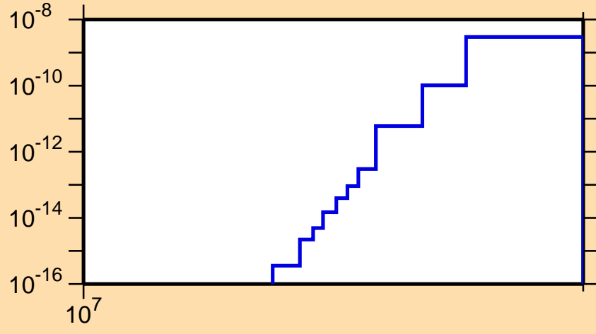
\sigma vs. E for ^{210}\text{Ra}(n,\text{pt})
