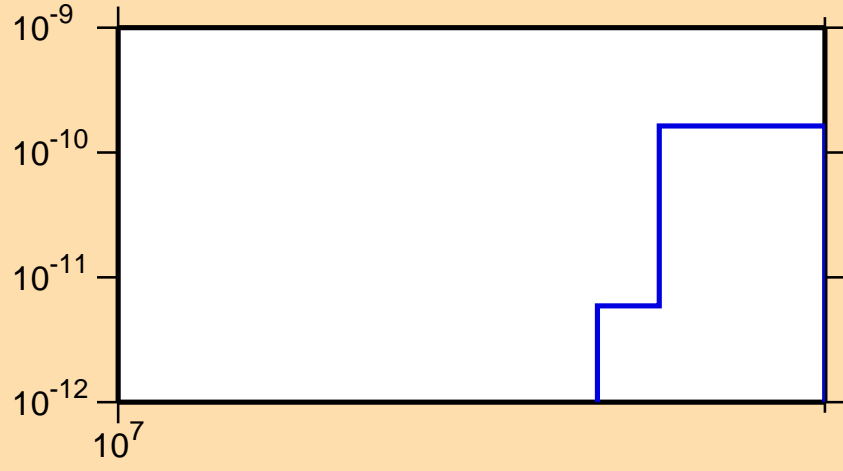
\sigma vs. E for ^{210}\text{Ra} (mt 34)
