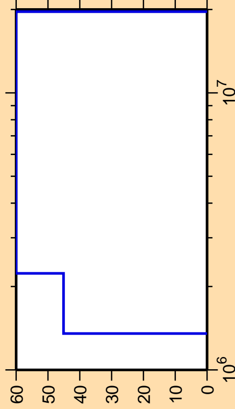
\Delta\sigma/\sigma vs. E for ^{210}\text{Ra}(n,n_4)
