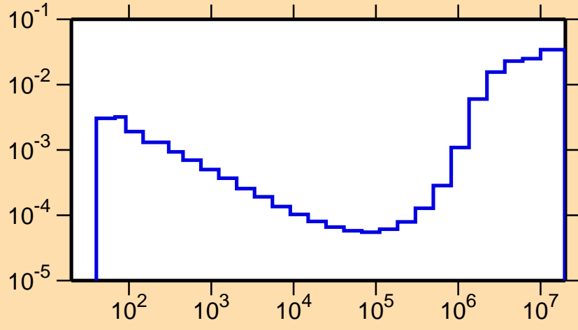
\sigma vs. E for ^{210}\text{Ra}(n,p)
