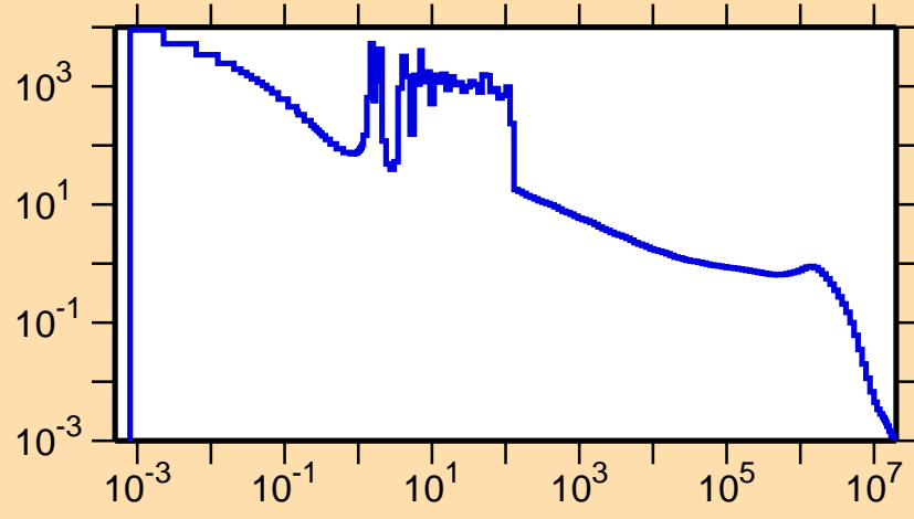
\sigma vs. E for ^{211}\text{Ra}(n,\gamma)
