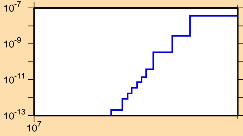
\sigma vs. E for ^{211}\text{Ra}(n,\text{pt})
