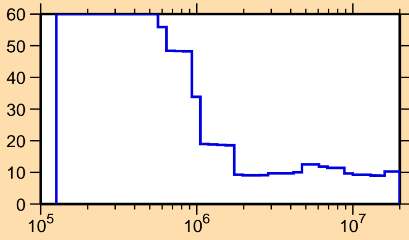
\Delta\sigma/\sigma vs. E for ^{211}\text{Ra}(n,\text{nonel.})
