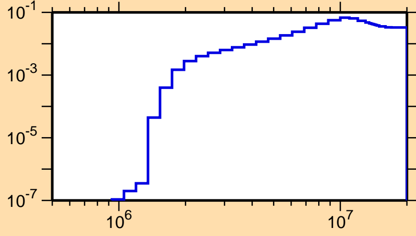
\sigma vs. E for ^{211}\text{Ra}(n,n\alpha)
