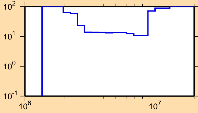
\Delta\sigma/\sigma vs. E for ^{211}\text{Ra}(n,n\text{cont.})
