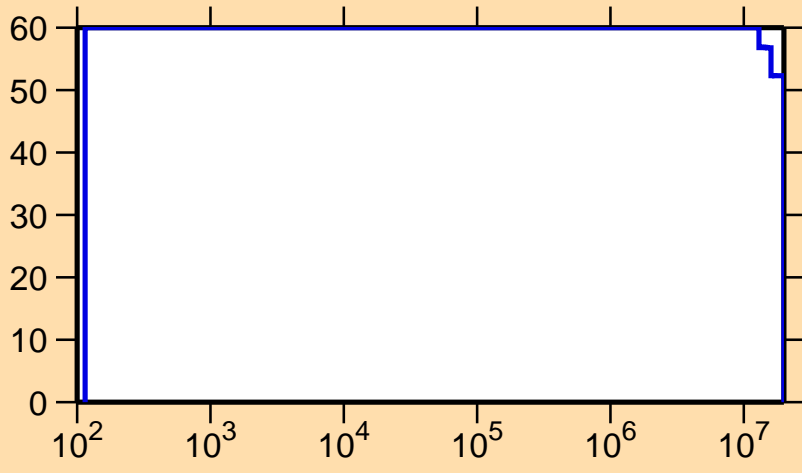
\Delta\sigma/\sigma vs. E for ^{211}\text{Ra}(n,p)
