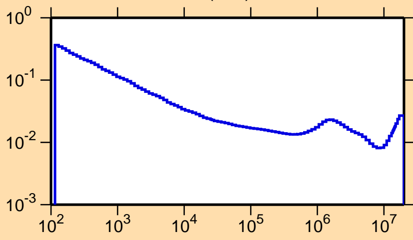
\sigma vs. E for ^{211}\text{Ra}(n,\alpha)
