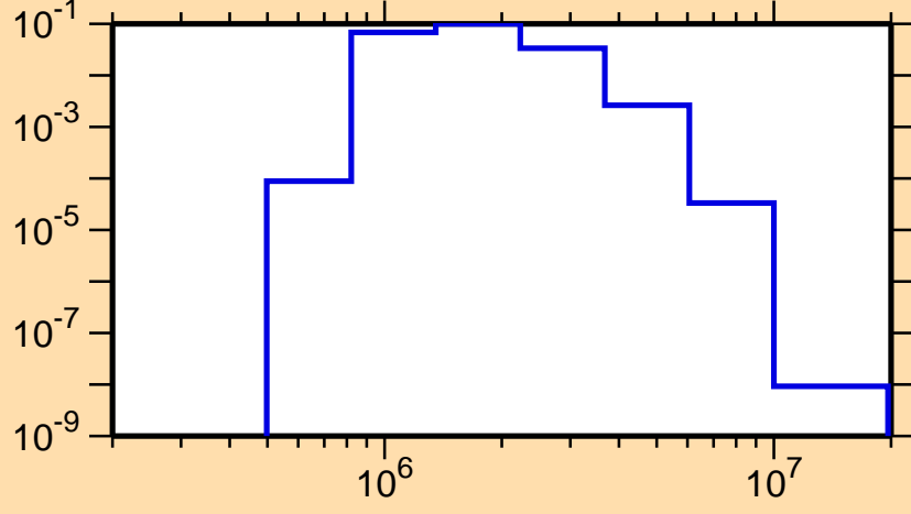
\sigma vs. E for ^{211}\text{Ra}(n,n_4)
