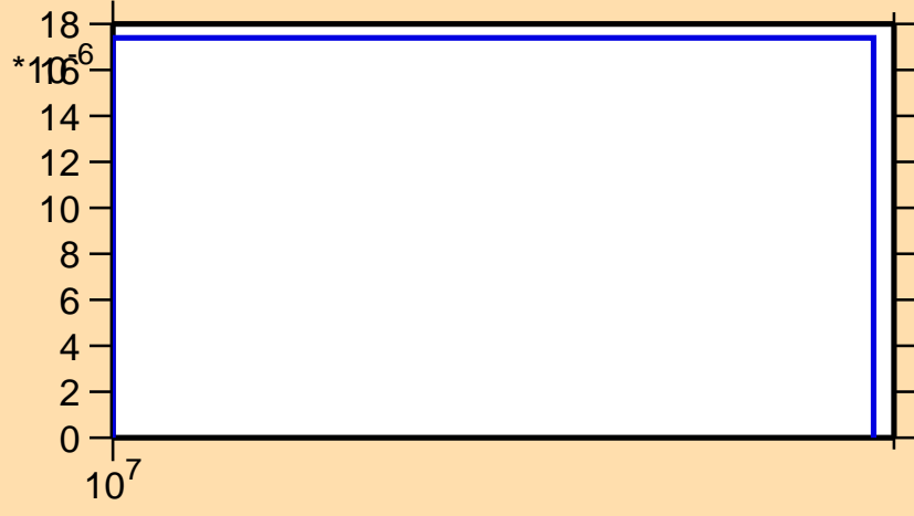
\sigma vs. E for ^{211}\text{Ra}(n,3n\alpha)
