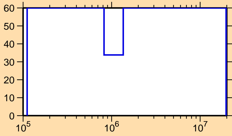
\Delta\sigma/\sigma vs. E for ^{211}\text{Ra}(n,n_1)
