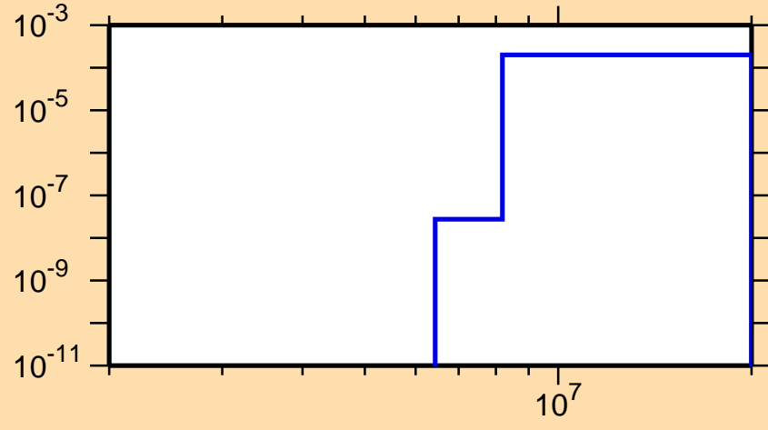
\sigma vs. E for ^{211}\text{Ra} (mt 45)
