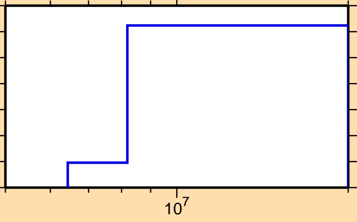
\sigma vs. E for ^{211}\text{Ra}(\text{mt117})
