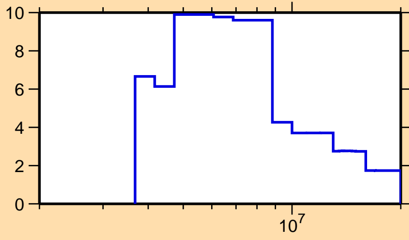
\Delta\sigma/\sigma vs. E for ^{212}\text{Ra}(n,\text{tot.})
