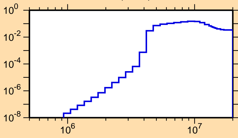
\sigma vs. E for ^{212}\text{Ra}(n,n\alpha)
