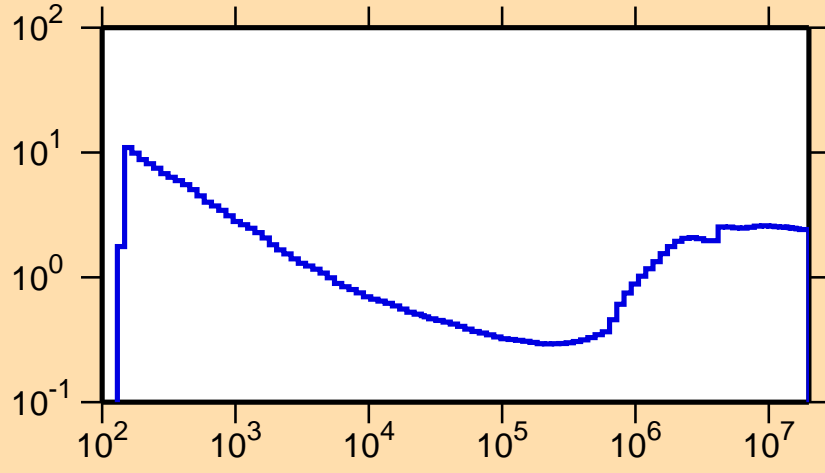
\sigma vs. E for ^{212}\text{Ra}(n,\text{nonel.})
