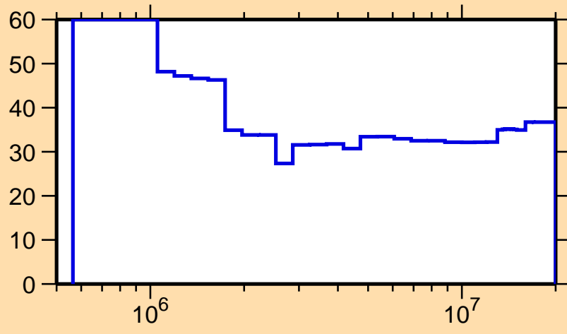
\Delta\sigma/\sigma vs. E for ^{212}\text{Ra}(n,n_1)
