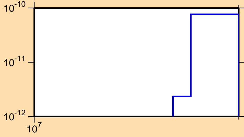
\sigma vs. E for ^{212}\text{Ra} (mt 34)
