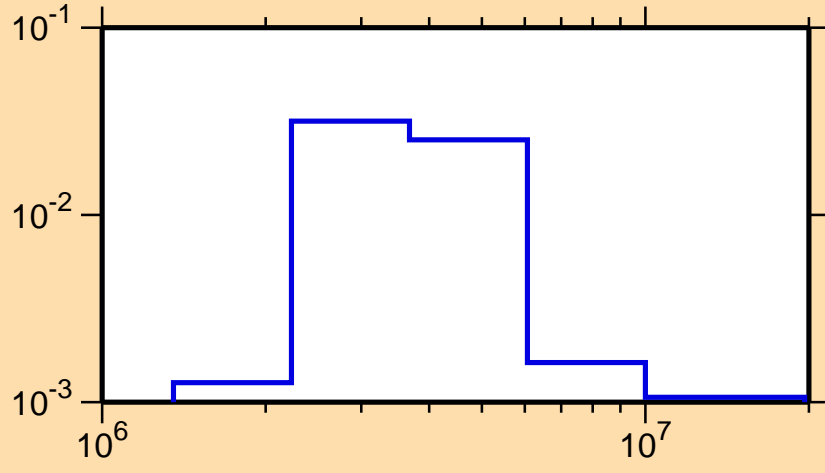
\sigma vs. E for ^{212}\text{Ra}(n,n_3)
