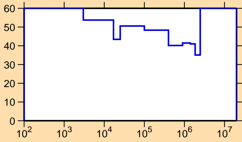
\Delta\sigma/\sigma vs. E for ^{212}\text{Ra}(n,\gamma)
