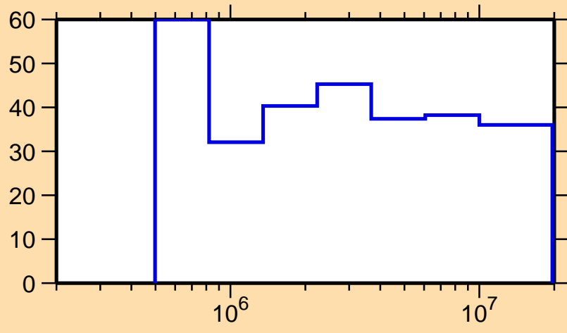
\Delta\sigma/\sigma vs. E for ^{213}\text{Ra}(n,n_1)
