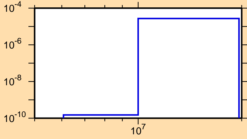
\sigma vs. E for ^{213}\text{Ra}(\text{mt117})
