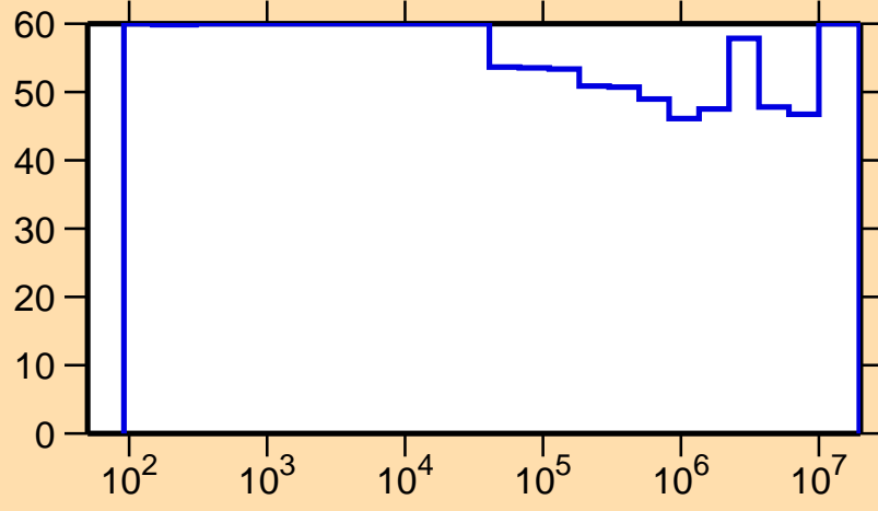
\Delta\sigma/\sigma vs. E for ^{213}\text{Ra}(n,\gamma)
