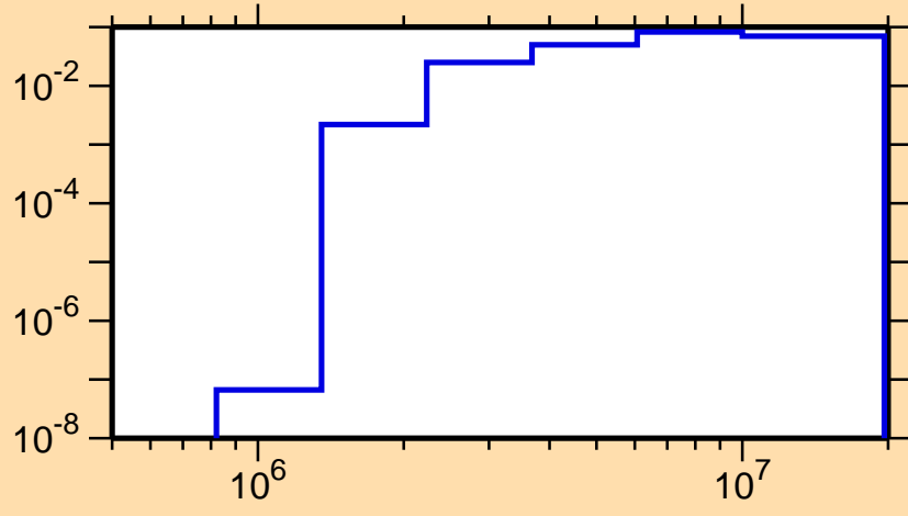
\sigma vs. E for ^{213}\text{Ra}(n,n\alpha)
