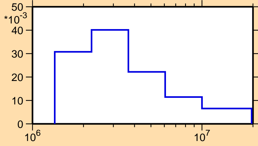
\sigma vs. E for ^{213}\text{Ra}(n,n_3)
