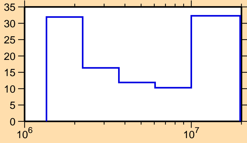
\Delta\sigma/\sigma vs. E for ^{213}\text{Ra}(n,n\text{cont.})
