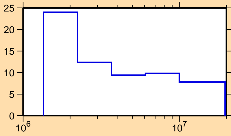
\Delta\sigma/\sigma vs. E for ^{213}\text{Ra}(n,n\text{onel.})
