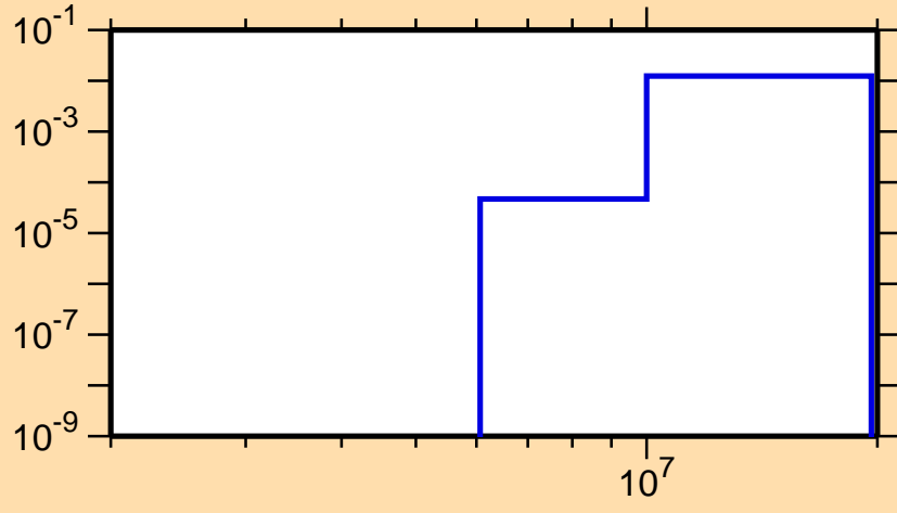
\sigma vs. E for ^{213}\text{Ra}(n,np)
