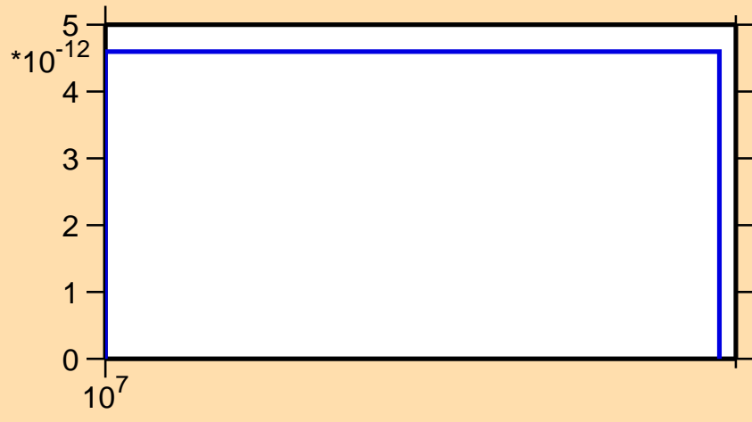
\sigma vs. E for ^{213}\text{Ra}(\text{mt } 34)
