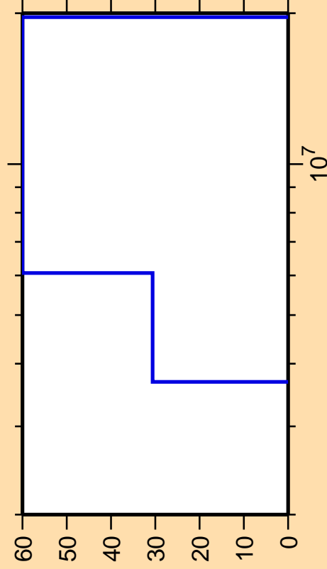
\Delta\sigma/\sigma vs. E for ^{213}\text{Ra}(n,np)
