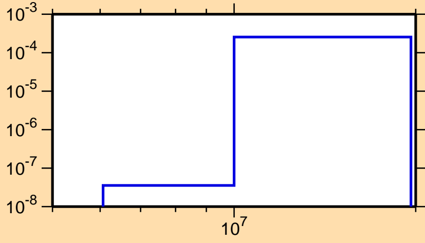
\sigma vs. E for ^{213}\text{Ra} (mt 45)
