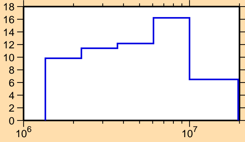
\Delta\sigma/\sigma vs. E for ^{213}\text{Ra}(n, el.)
