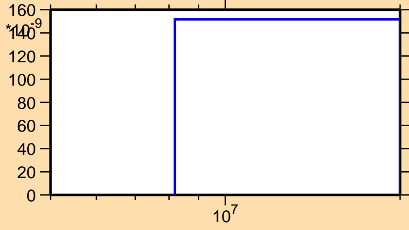
\sigma vs. E for ^{213}\text{Ra}(n,\text{He3})
