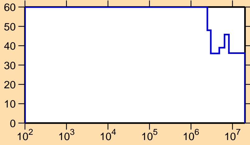
\Delta\sigma/\sigma vs. E for ^{213}\text{Ra}(n,p)
