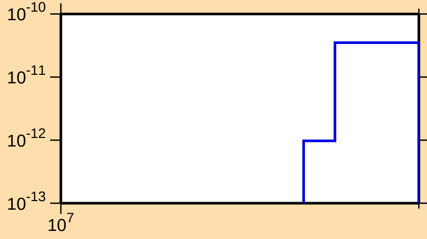
\sigma vs. E for ^{214}\text{Ra}(\text{mt } 34)
