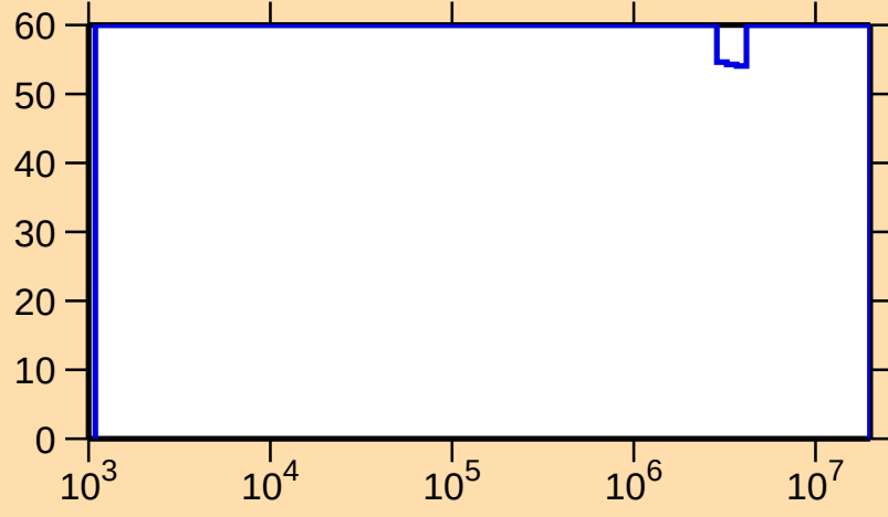
\Delta\sigma/\sigma vs. E for ^{214}\text{Ra}(n,\gamma)
