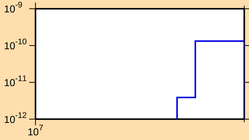
\sigma vs. E for ^{214}\text{Ra}(n,\text{pt})
