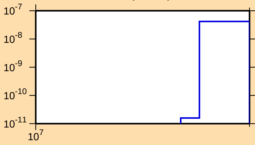
\sigma vs. E for ^{214}\text{Ra}(n,3n\alpha)
