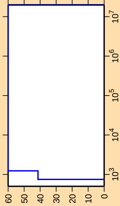
\Delta\sigma/\sigma vs. E for ^{214}\text{Ra}(n,\alpha)
