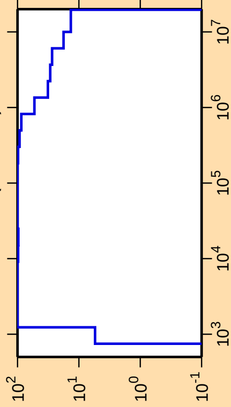
\Delta\sigma/\sigma vs. E for ^{214}\text{Ra}(n,\text{nonel.})
