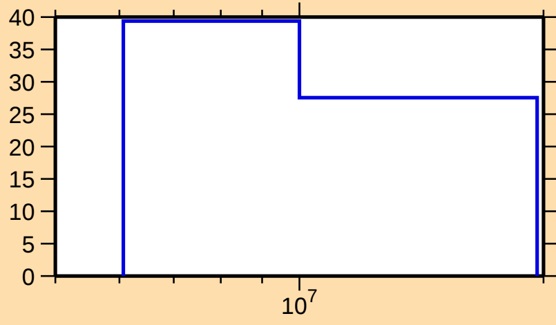
\Delta\sigma/\sigma vs. E for ^{214}\text{Ra}(n,2n)
