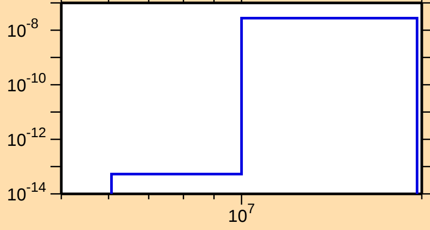
\sigma vs. E for ^{214}\text{Ra}(n,\text{He}3)
