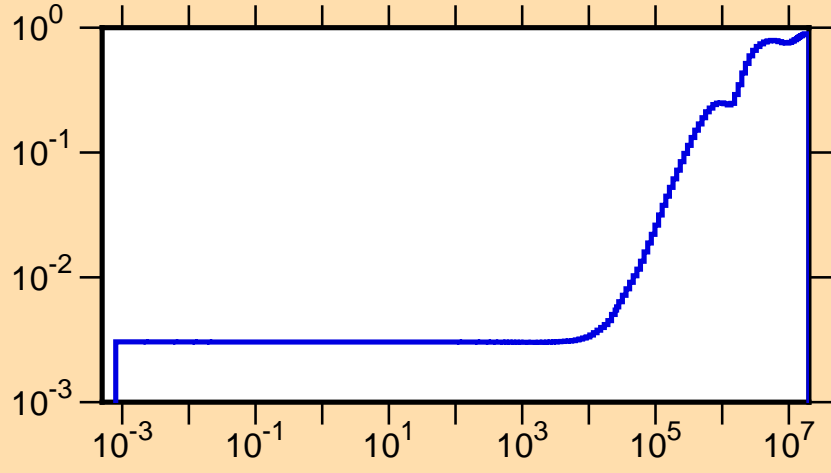
\mu vs. E for ^{221}\text{Ra}(\text{mt251})
