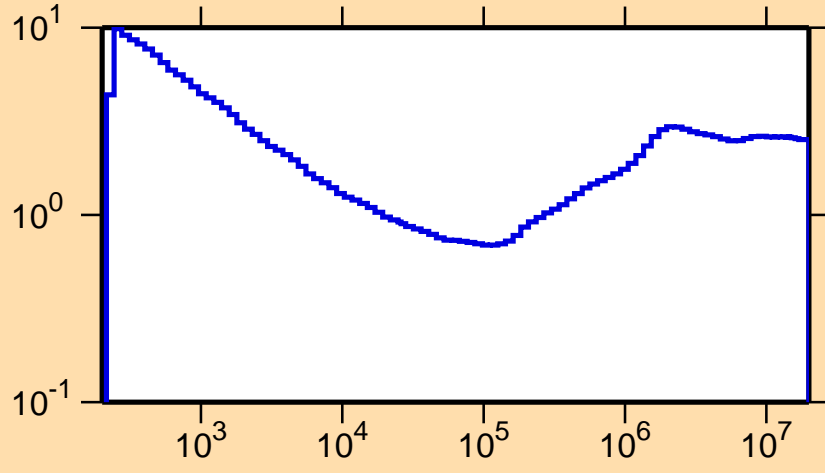
\sigma vs. E for ^{221}\text{Ra}(n,\text{nonel.})
