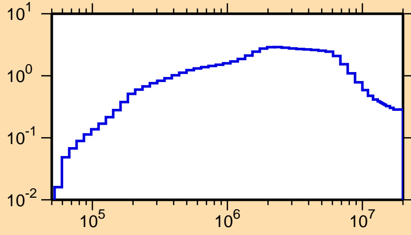
\sigma vs. E for ^{221}\text{Ra}(n,\text{inel.})
