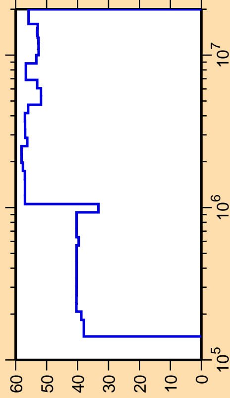
\Delta\sigma/\sigma vs. E for ^{221}\text{Ra}(n,n_4)
