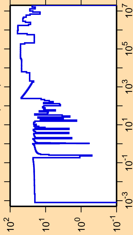
\Delta\sigma/\sigma vs. E for ^{221}\text{Ra}(n,\text{el.})
