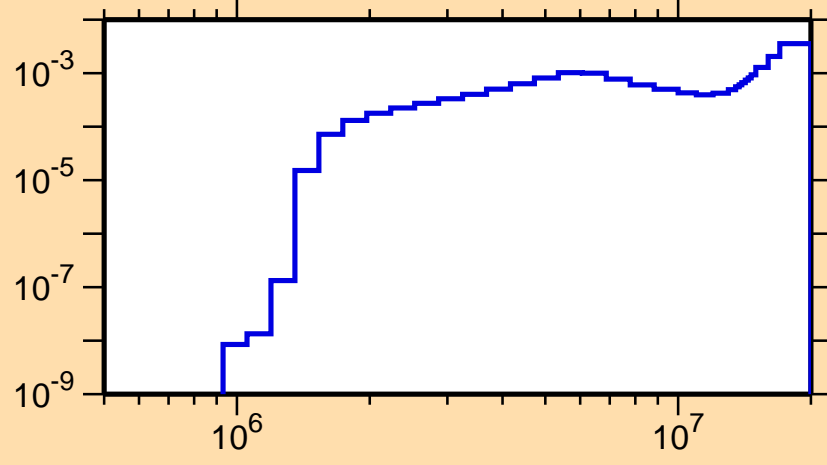
\sigma vs. E for ^{221}\text{Ra}(n,n\alpha)
