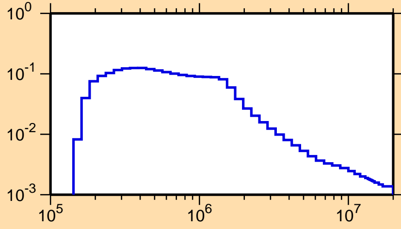
\sigma vs. E for ^{221}\text{Ra}(n,n_4)
