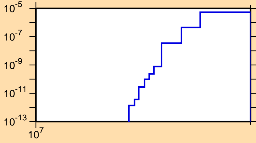
\sigma vs. E for ^{221}\text{Ra}(n,2np)
