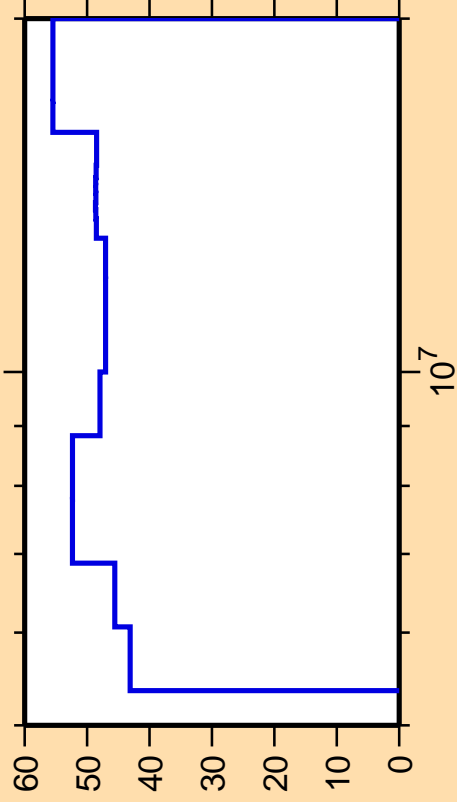
\Delta\sigma/\sigma vs. E for ^{221}\text{Ra}(n,n_1)
