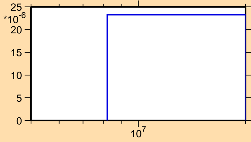
\sigma vs. E for ^{221}\text{Ra}(\text{mt } 45)
