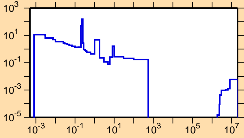
\sigma vs. E for ^{221}\text{Ra}(n,f)
