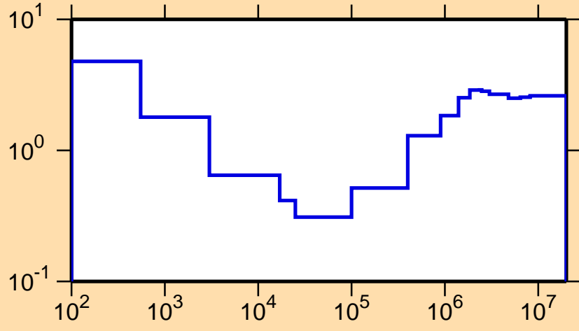
\sigma vs. E for ^{222}\text{Ra}(n,\text{nonel.})
