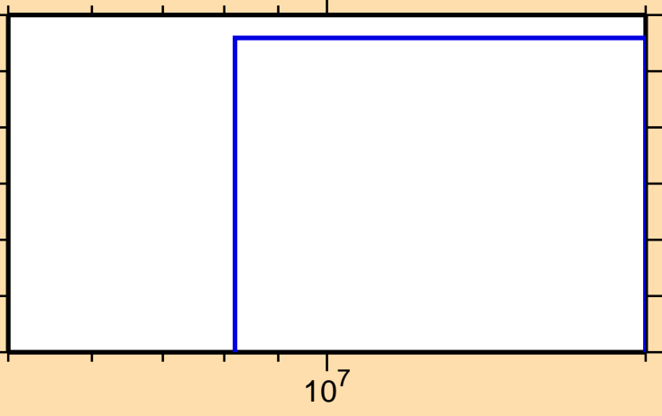
\sigma vs. E for ^{222}\text{Ra}(n,\text{nd})
