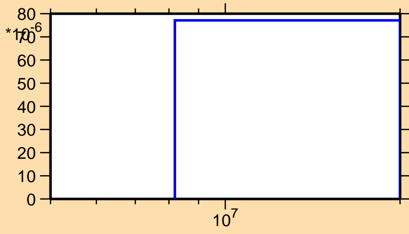
\sigma vs. E for ^{222}\text{Ra}(n,d)
