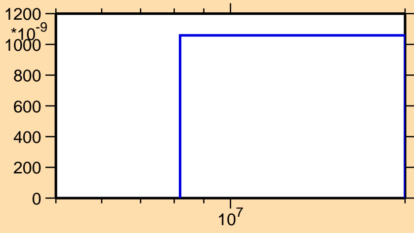
\sigma vs. E for ^{222}\text{Ra} (mt 45)
