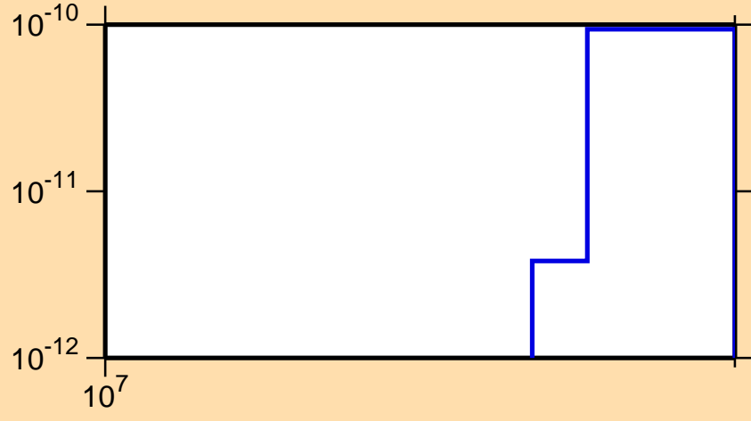
\sigma vs. E for ^{223}\text{Ra}(n,\text{He}3)
