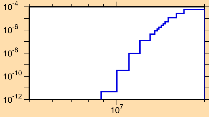
\sigma vs. E for ^{223}\text{Ra}(\text{mt117})
