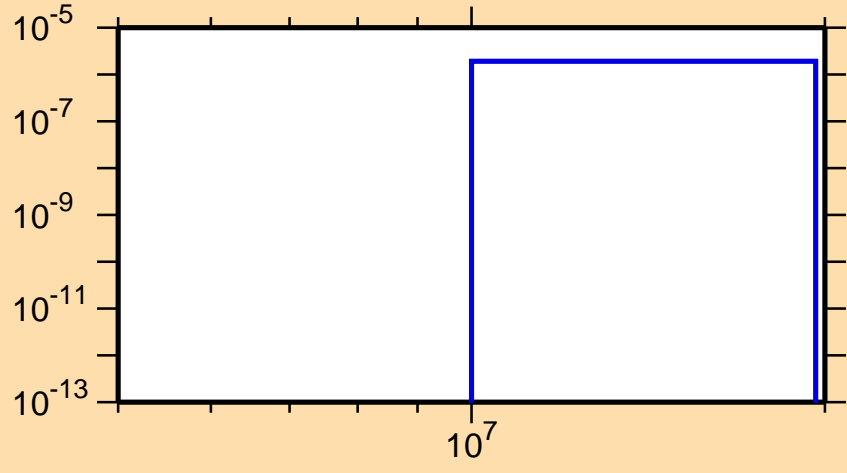
\sigma vs. E for ^{223}\text{Ra} (mt 45)
