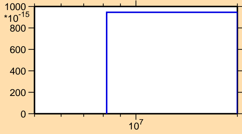
\sigma vs. E for ^{223}\text{Ra}(n,\text{He}3)
