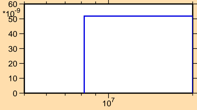
\sigma vs. E for ^{223}\text{Ra}(n,\text{nd})
