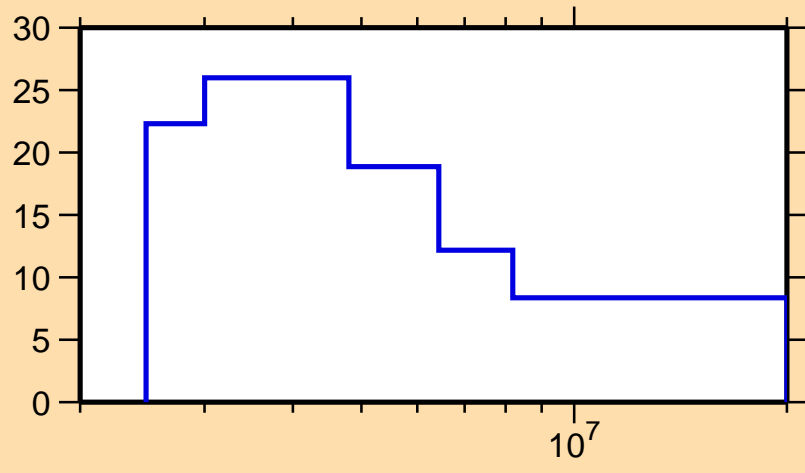
\Delta\sigma/\sigma vs. E for ^{223}\text{Ra}(n,\text{tot.})
