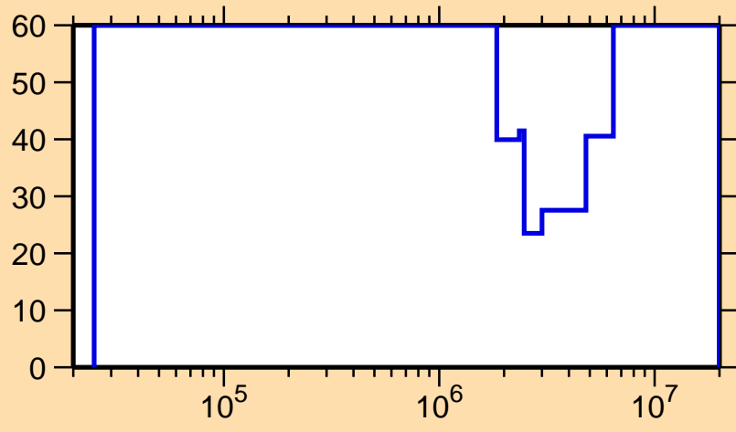
\Delta\sigma/\sigma vs. E for ^{223}\text{Ra}(n,\text{inel.})
