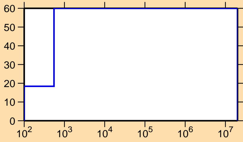
\Delta\sigma/\sigma vs. E for ^{223}\text{Ra}(n,\gamma)
