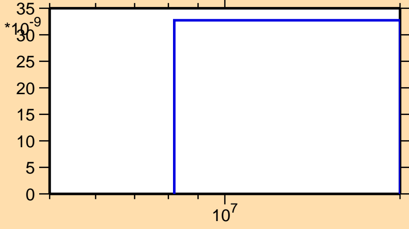
\sigma vs. E for ^{223}\text{Ra}(n,nt)
