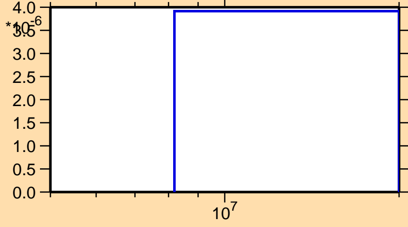
\sigma vs. E for ^{223}\text{Ra}(\text{mt117})
