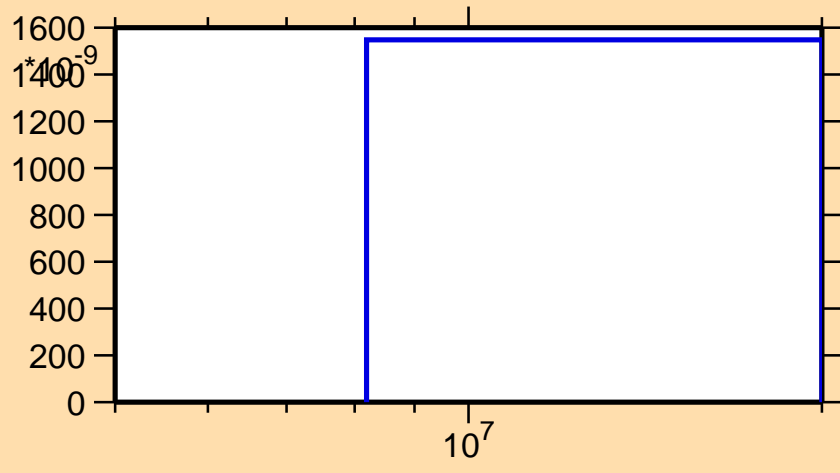
\sigma vs. E for ^{223}\text{Ra} (mt 45)
