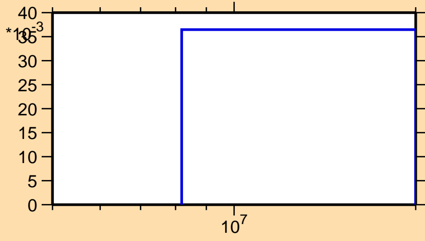
\sigma vs. E for ^{223}\text{Ra}(n,3n\alpha)
