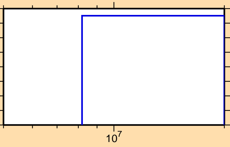
\sigma vs. E for ^{223}\text{Ra}(n,2np)
