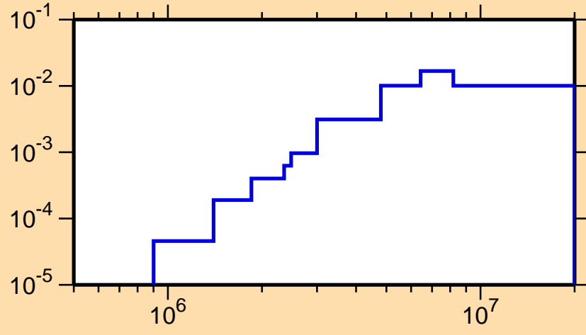
\sigma vs. E for ^{223}\text{Ra}(n,n\alpha)
