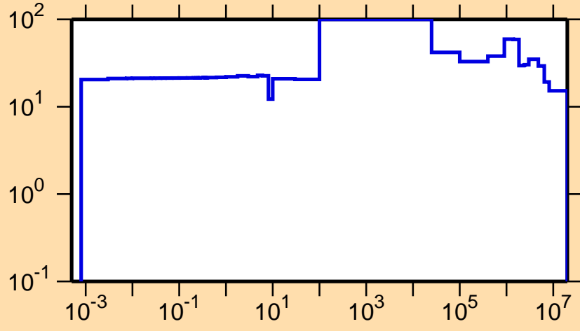
\Delta\sigma/\sigma vs. E for ^{223}\text{Ra}(n,el.)
