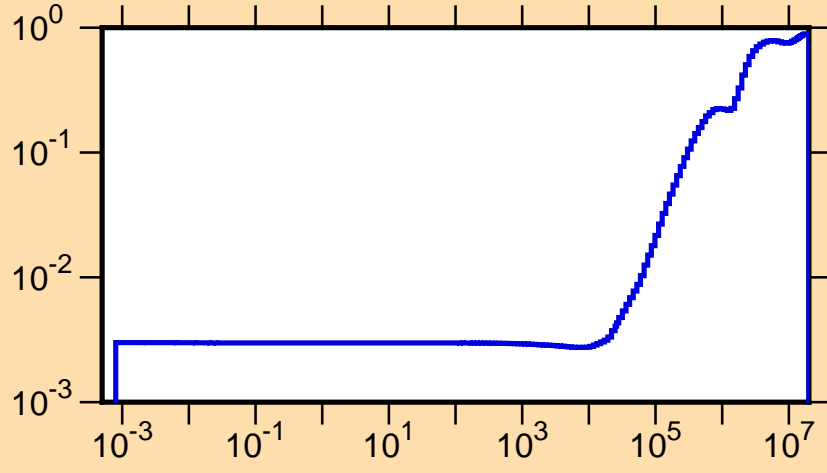
\mu vs. E for ^{224}\text{Ra}(\text{mt251})
